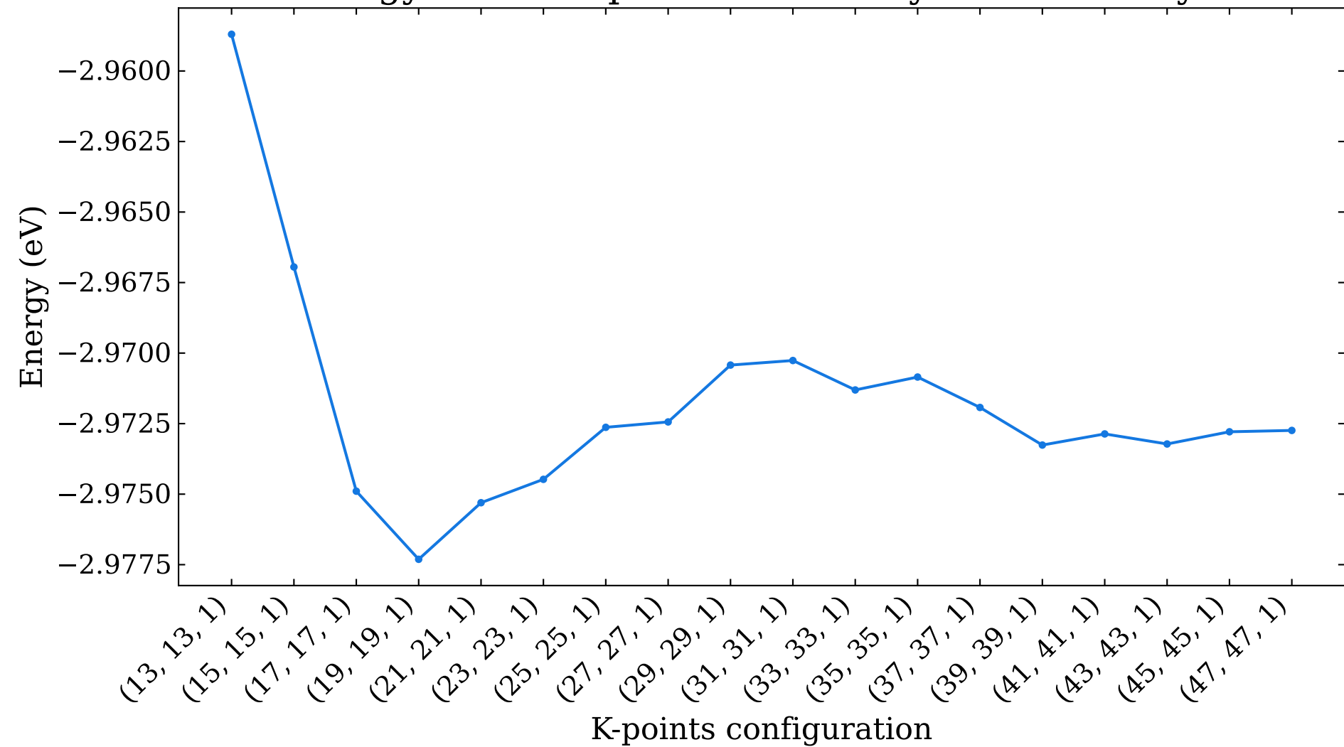
Energy versus k-points for \alpha -beryllene monolayer
