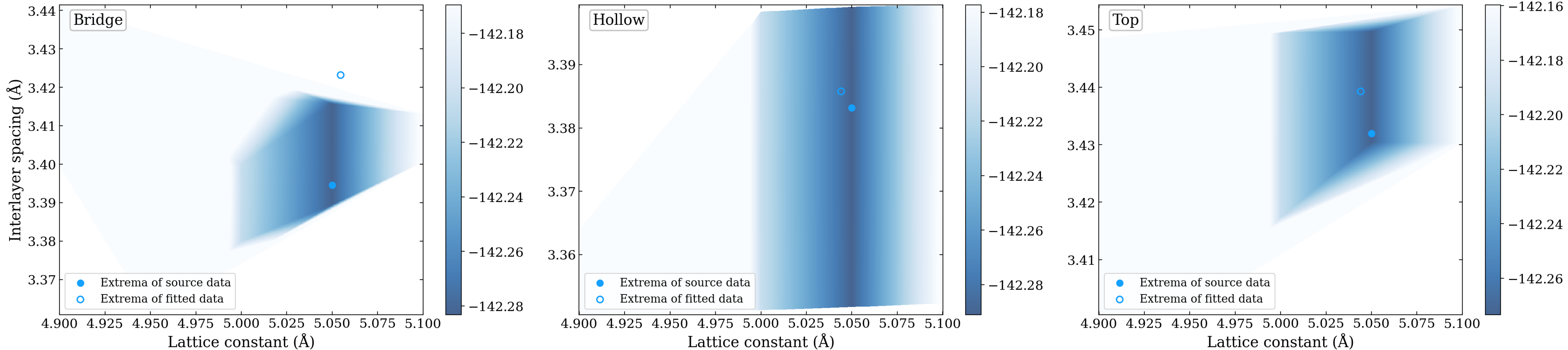
Free energy versus lattice and spacing for Graphene-BC 3
