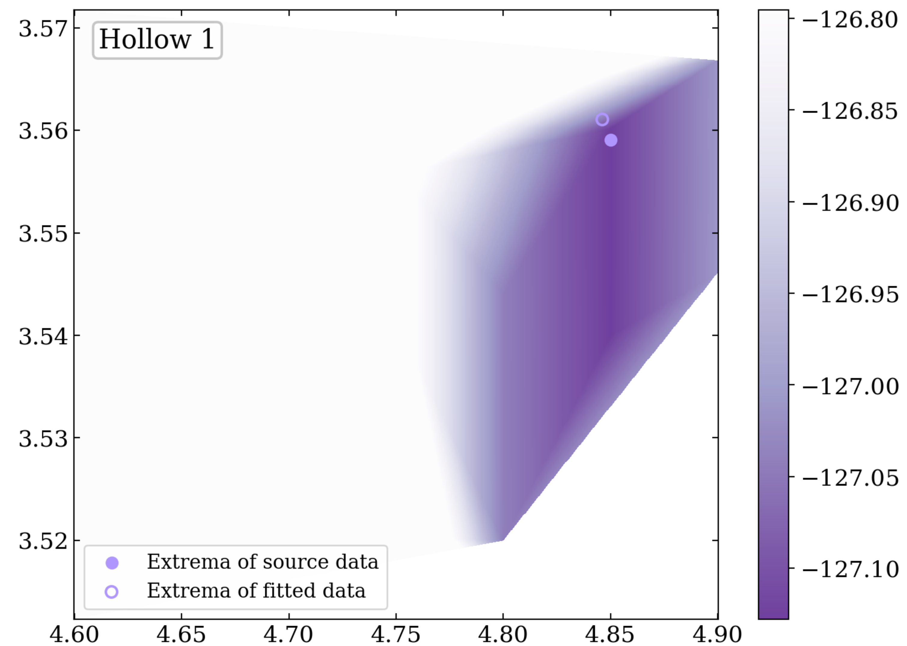
Free energy versus lattice and spacing for Graphene-B 4 C 3
