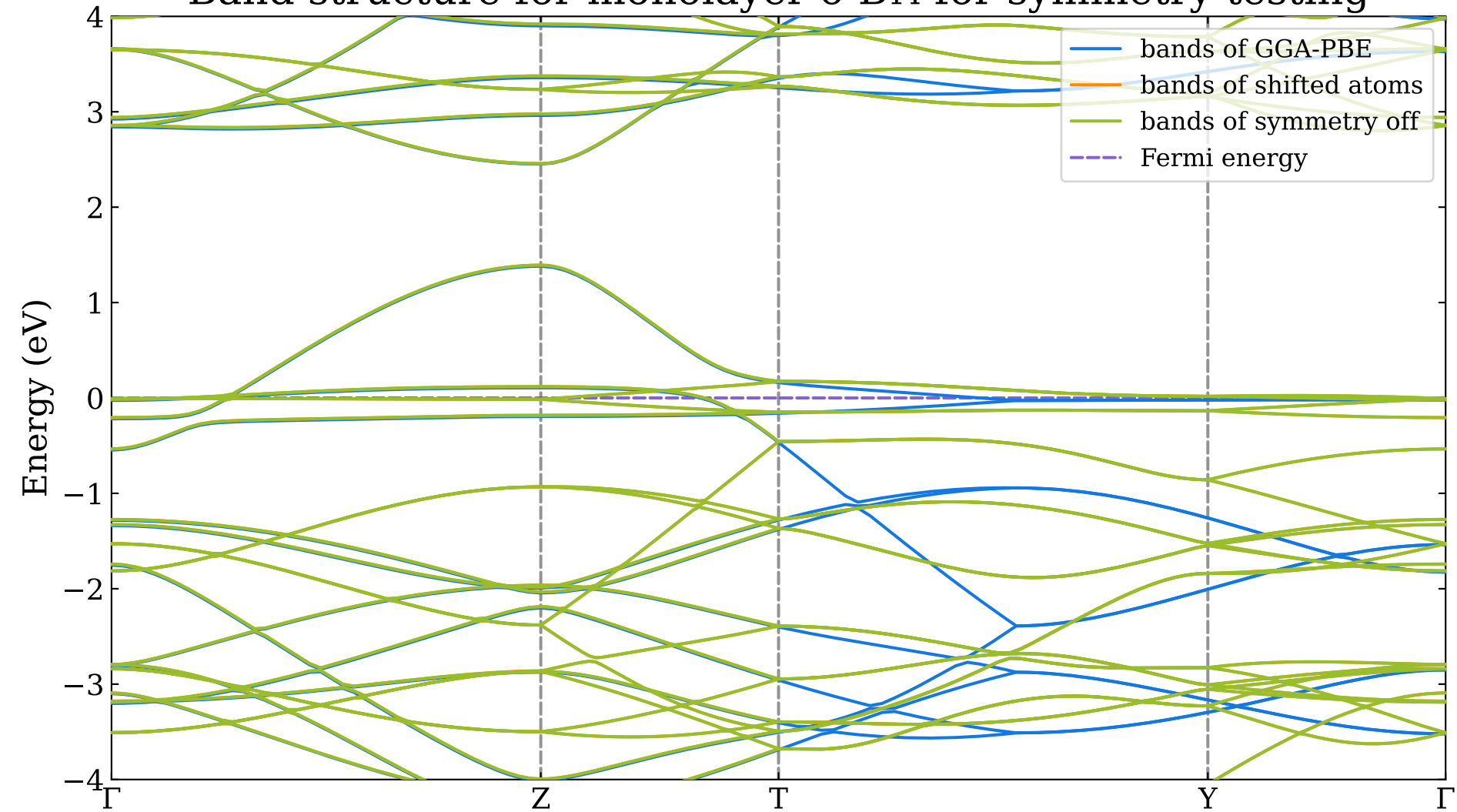
Band structure for monolayer o-B 14 for symmetry testing
