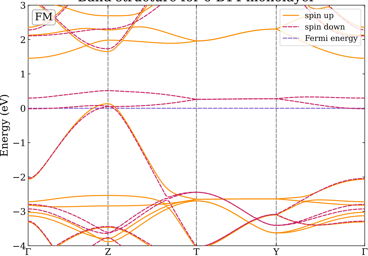
Band structure for o-B14 monolayer
