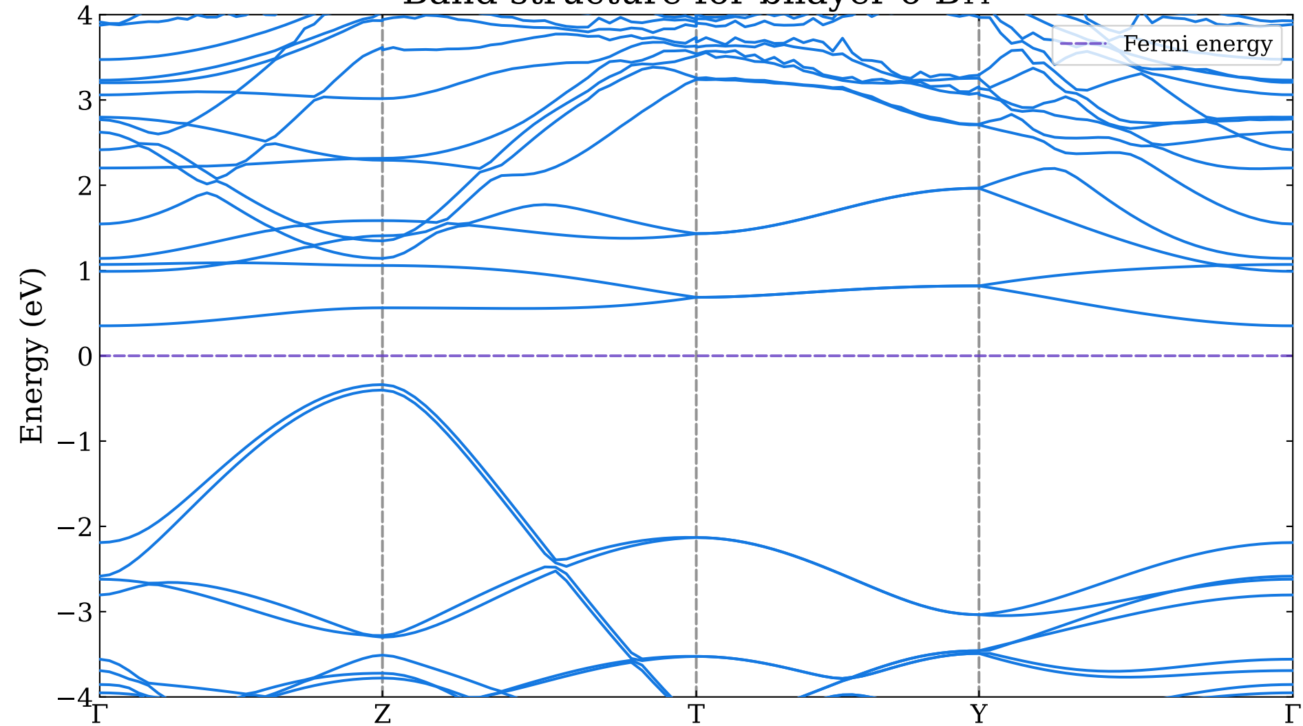
Band structure for bilayer o-B 14
