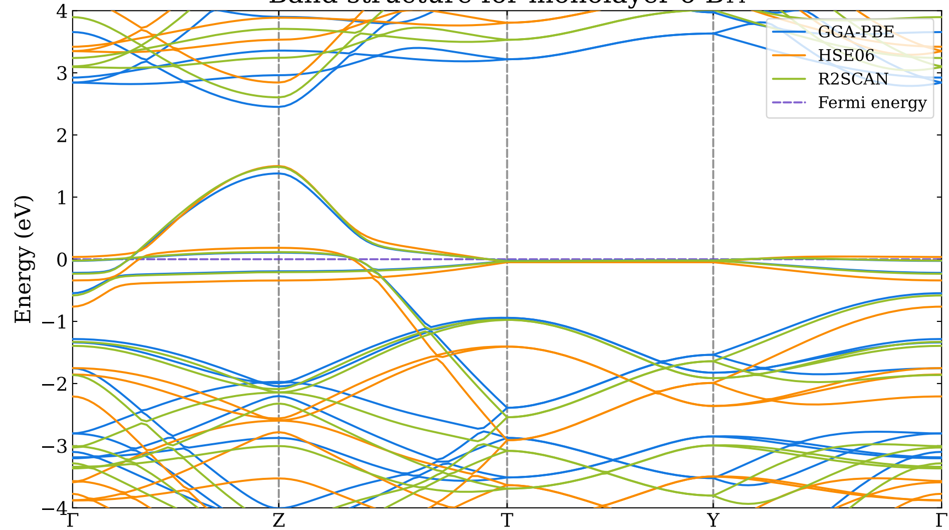
Band structure for monolayer o-B 14
