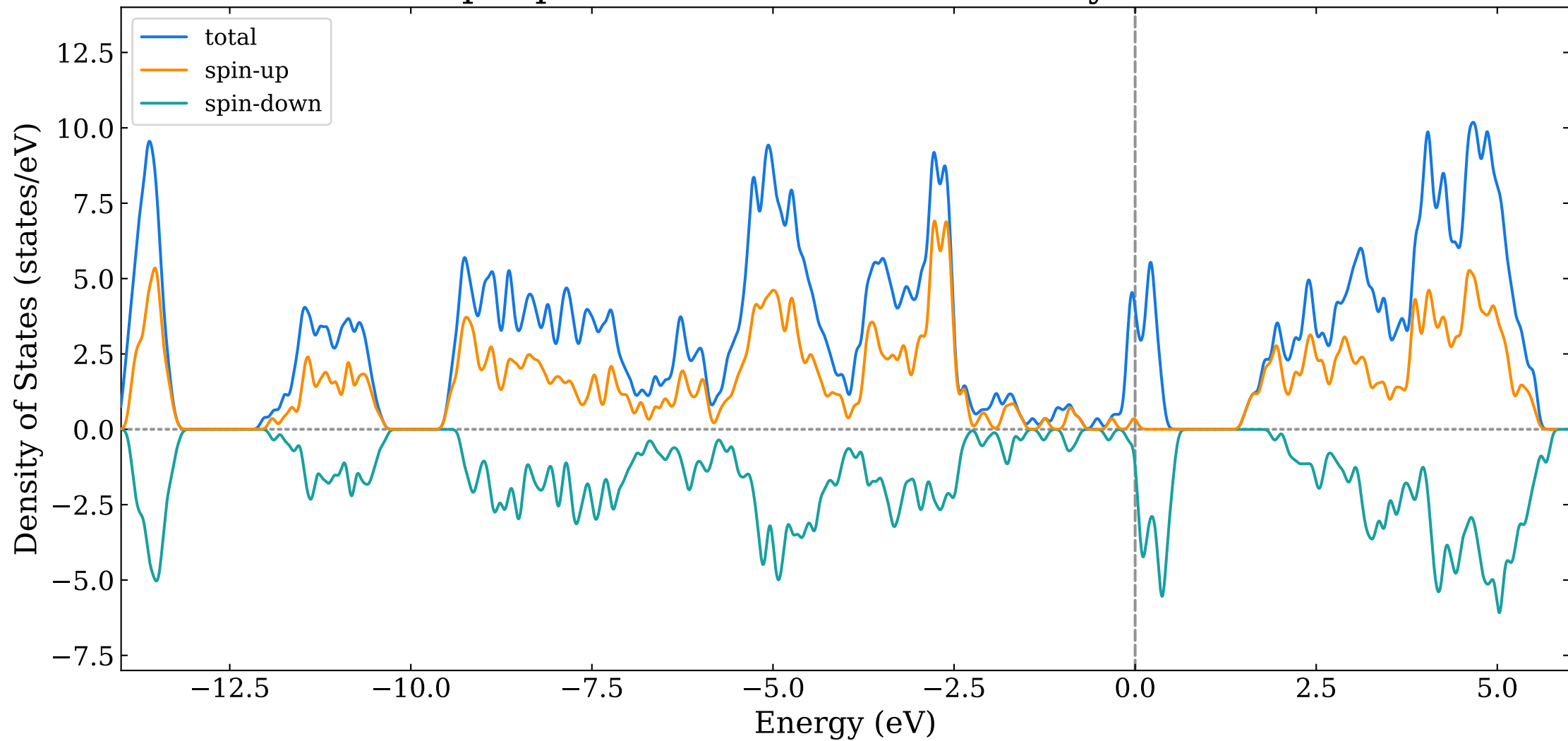
Spin-polarized DOS of FM monolayer o-B 14
