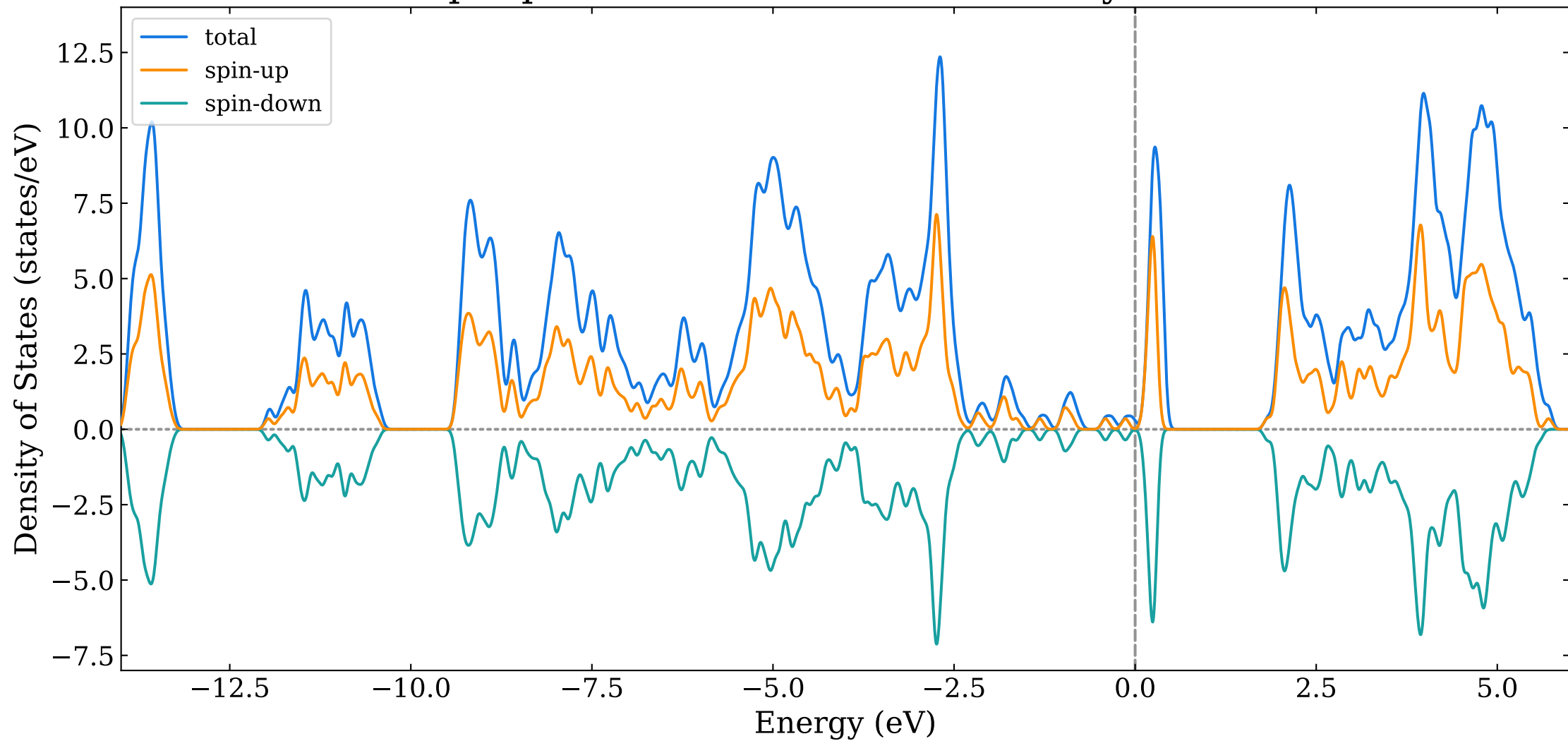
Spin-polarized DOS of AFM monolayer o-B 14
