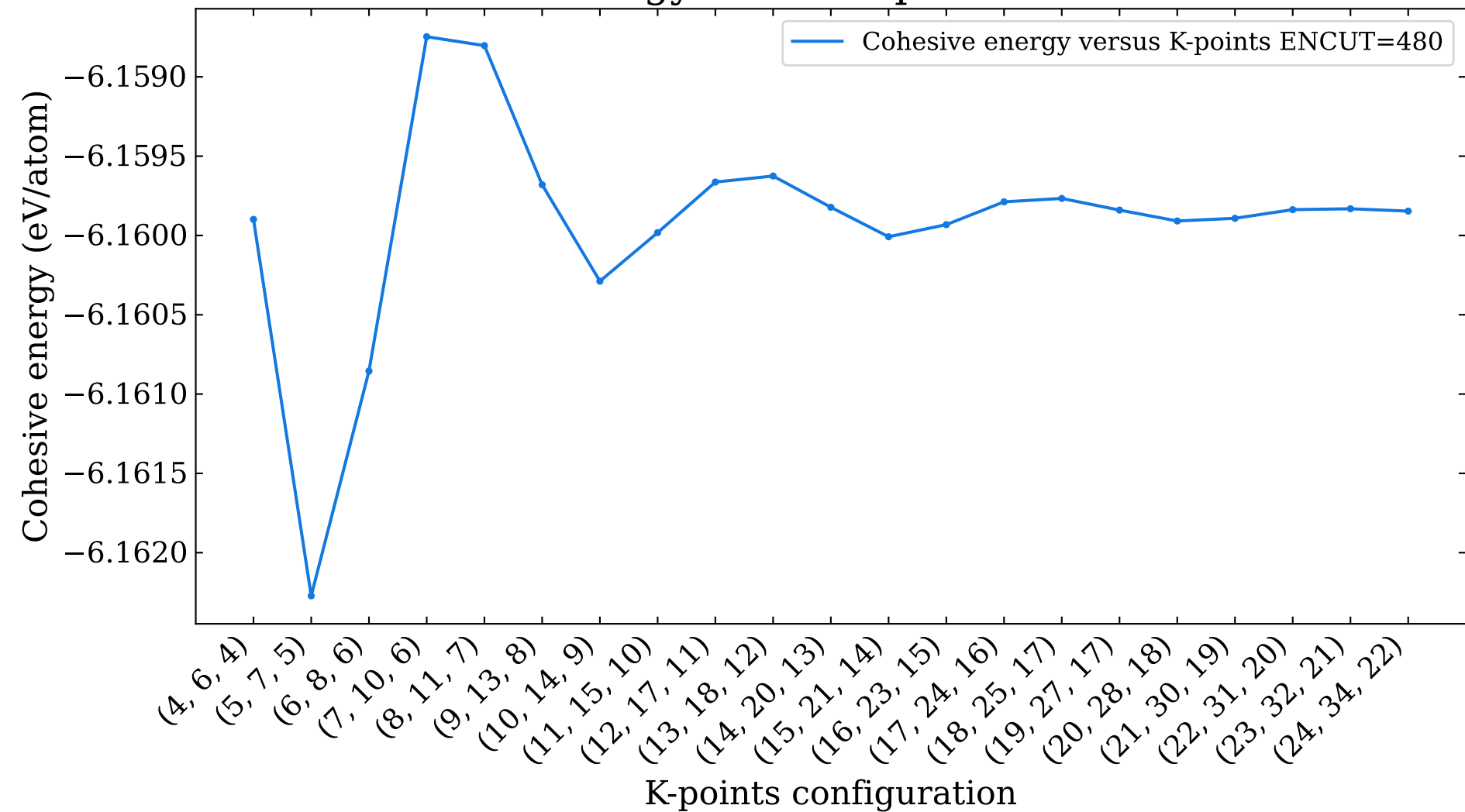
Cohesive energy versus k-points for o-B 14 bulk
