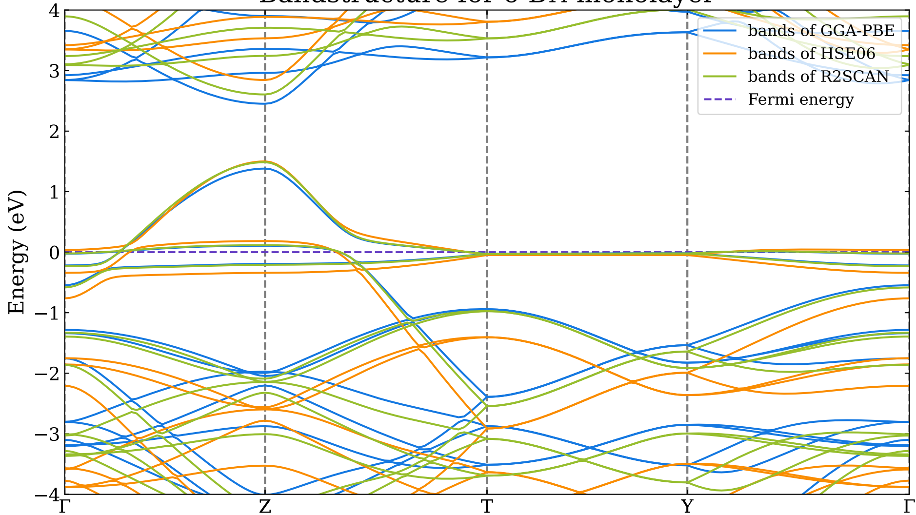
Bandstructure for o-B 14 monolayer
