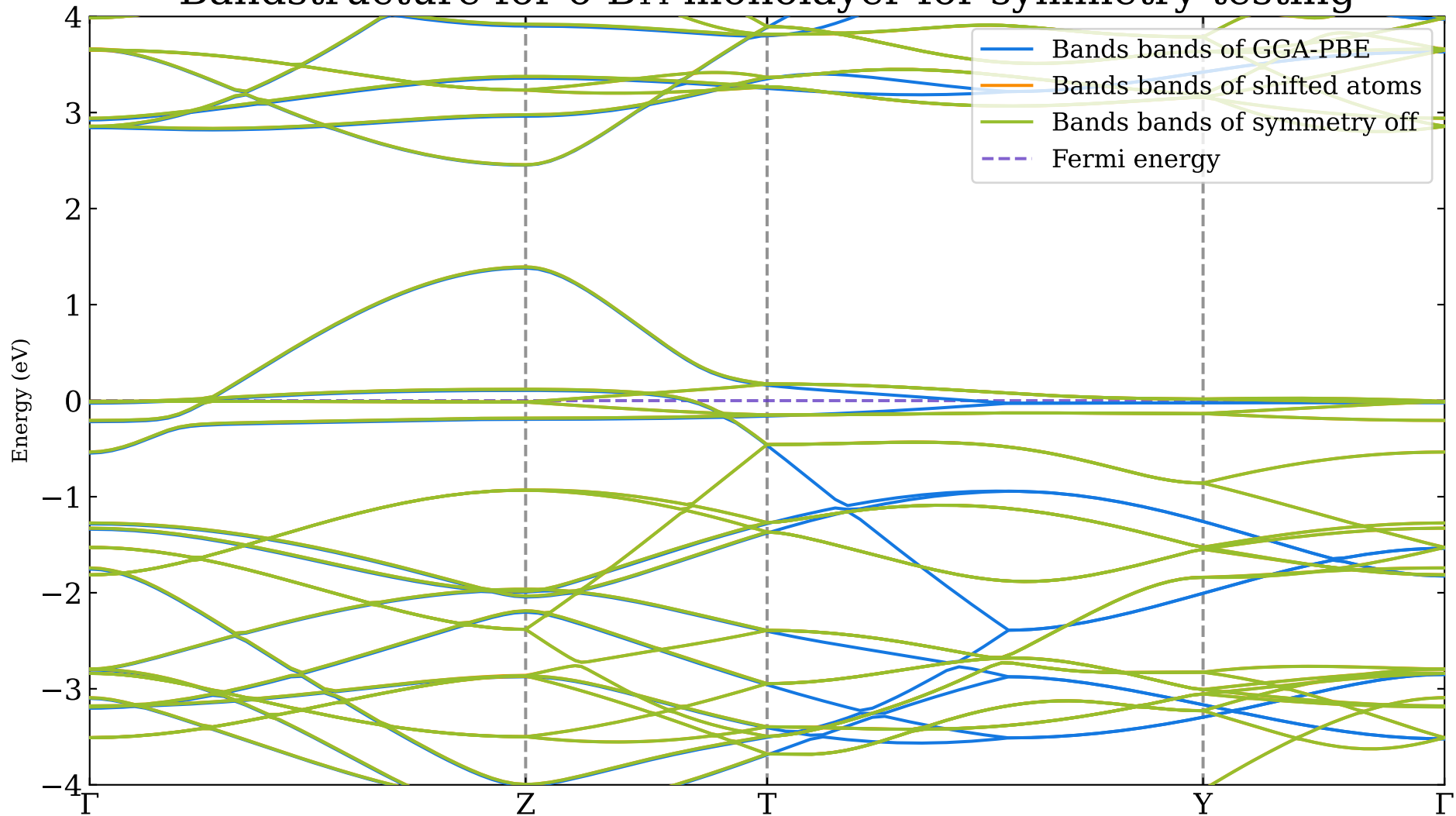
Bandstructure for o-B 14 monolayer for symmetry testing
