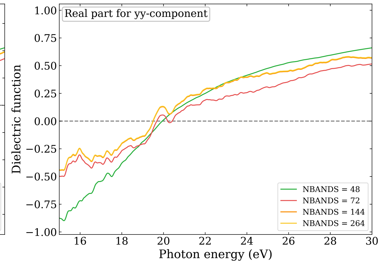
Dielectric function versus NBANDS for bulk o-B 14
