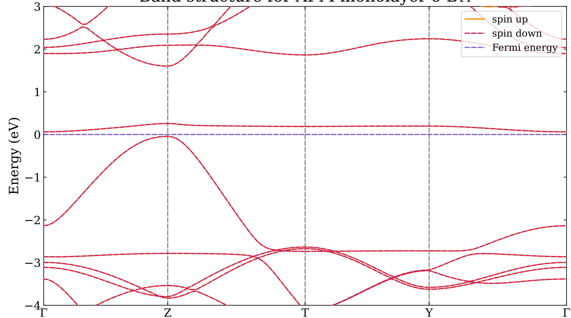
Band structure for AFM monolayer o-B 14
