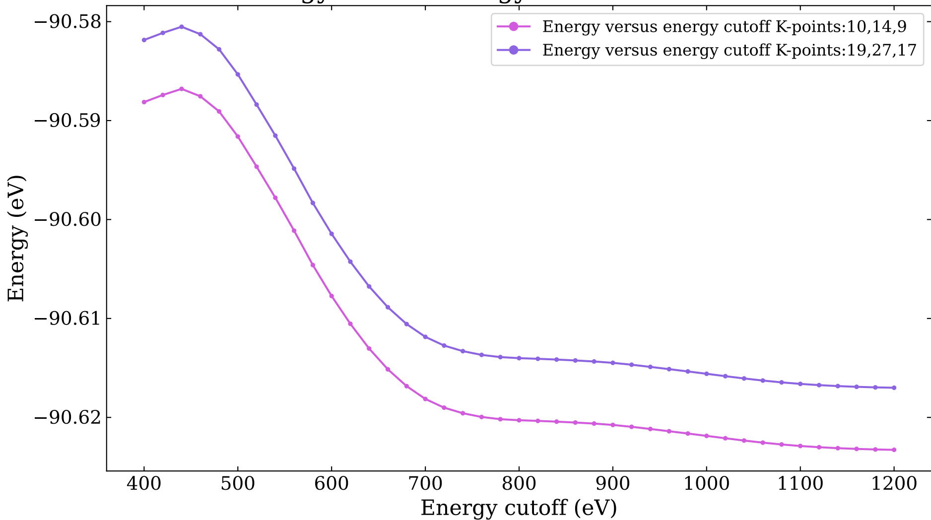
Energy versus energy cutoff for o-B 14 bulk
