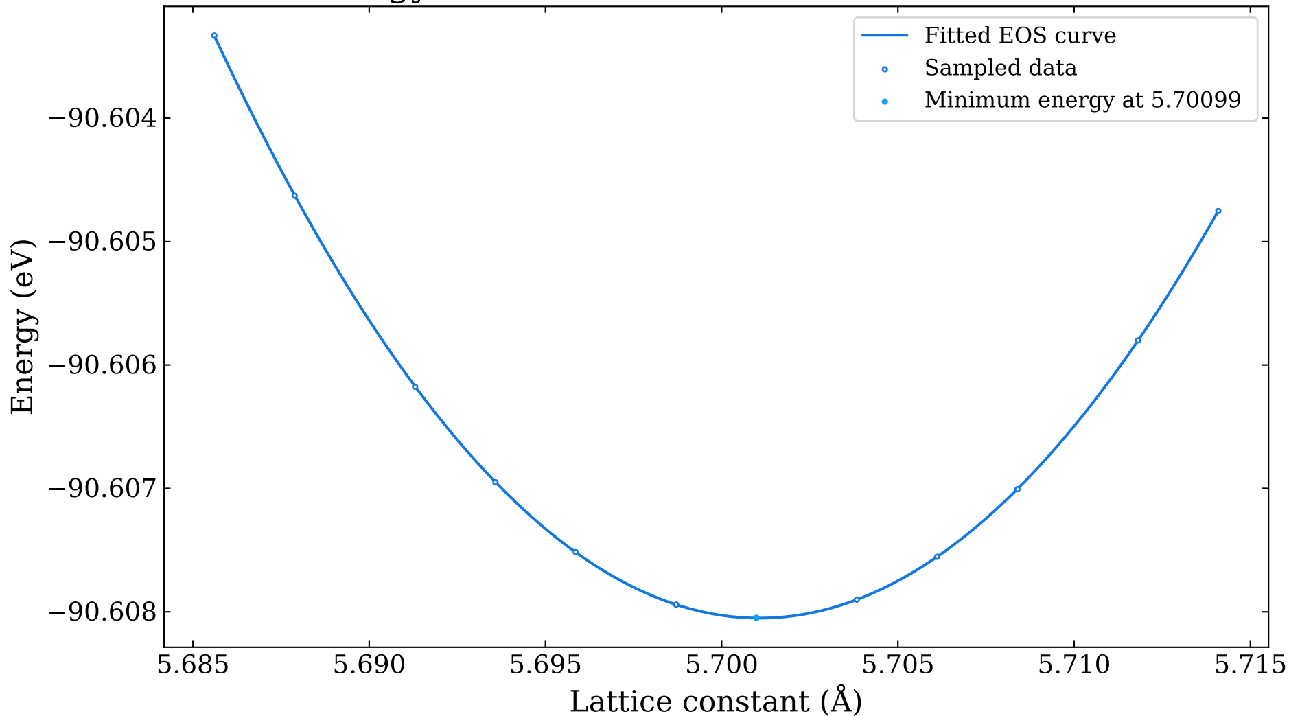
Energy versus lattice constant for o-B 14 bulk
