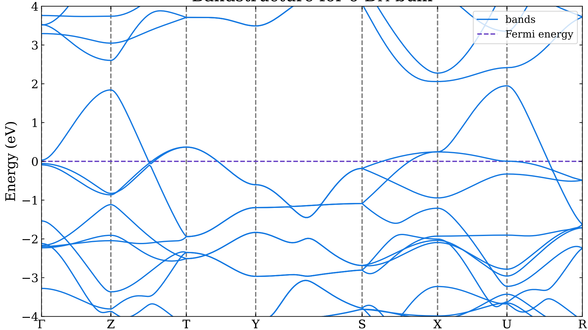
Bandstructure for o-B 14 bulk
