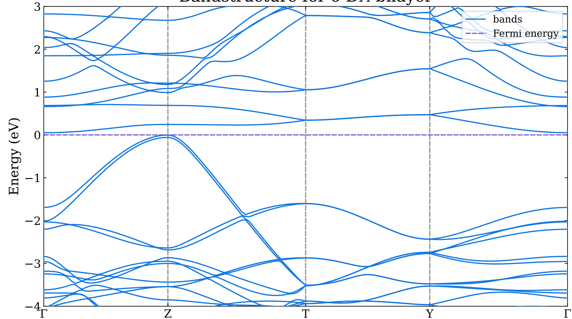
Bandstructure for o-B 14 bilayer
