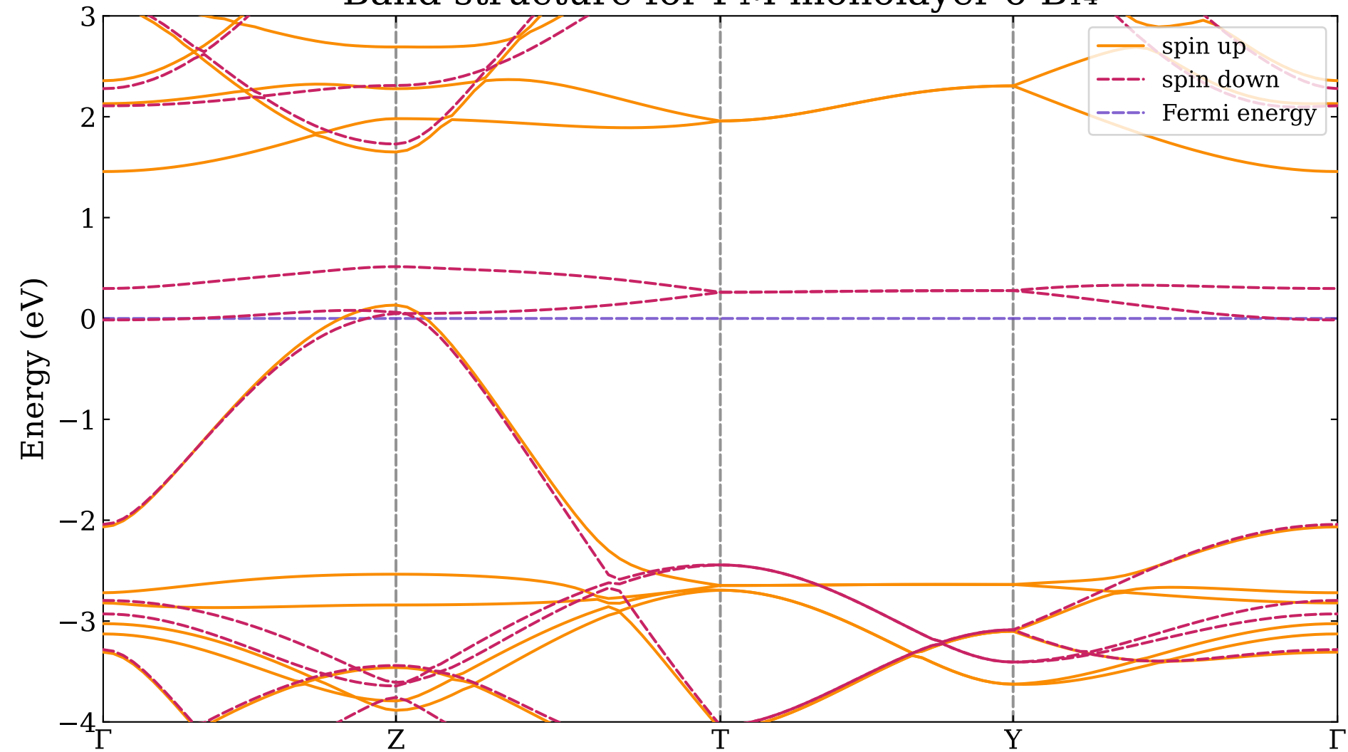
Band structure for FM monolayer o-B 14
