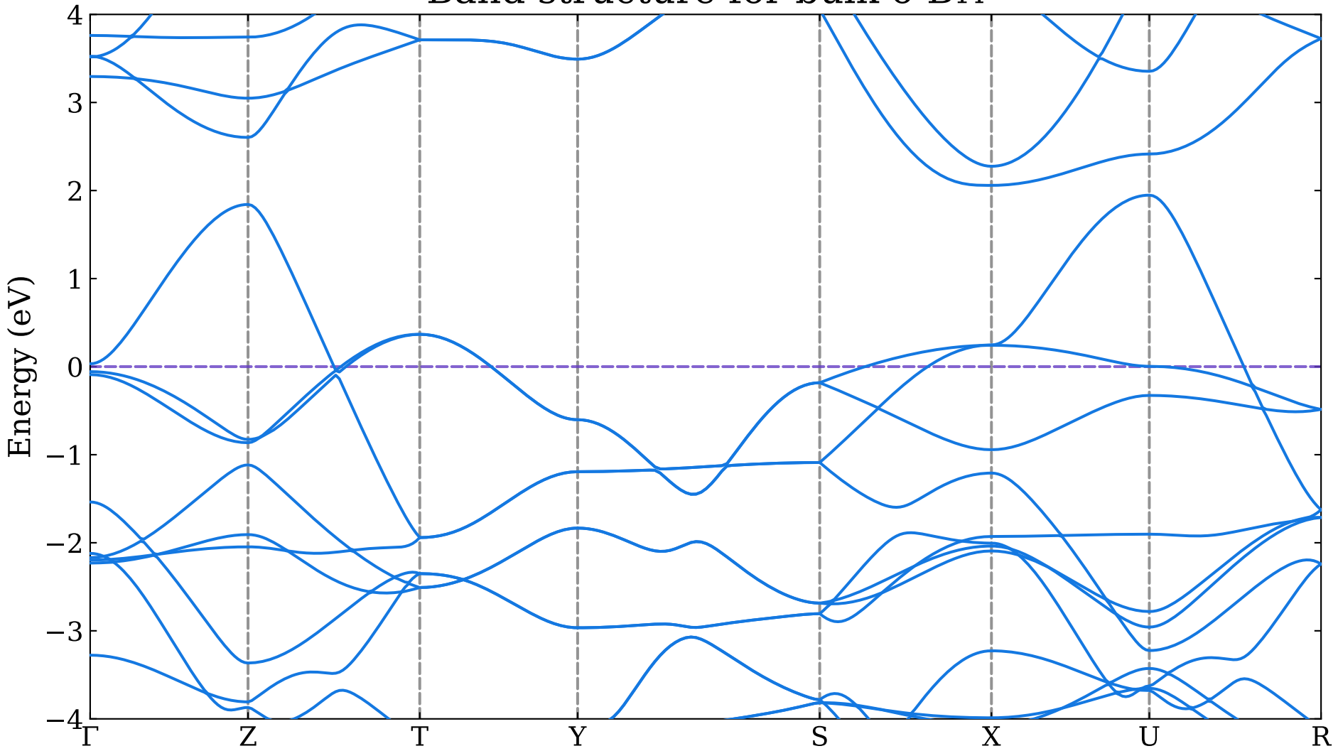
Band structure for bulk o-B 14
