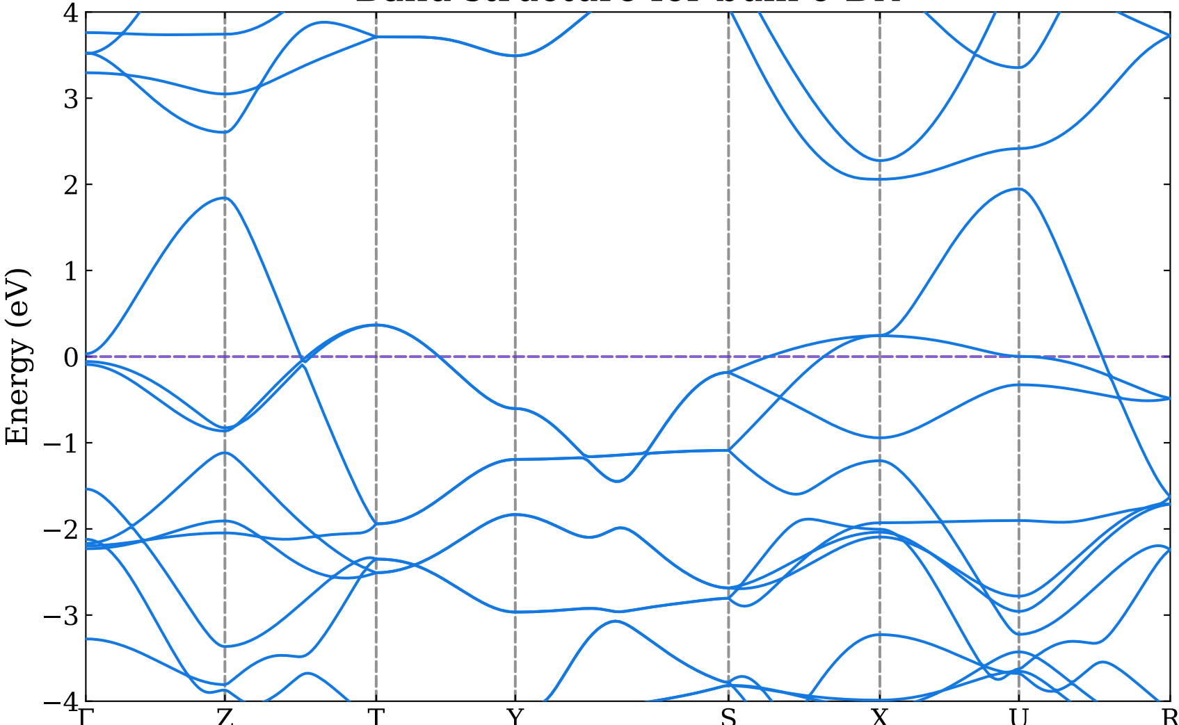
Band structure for bulk o-B 14
