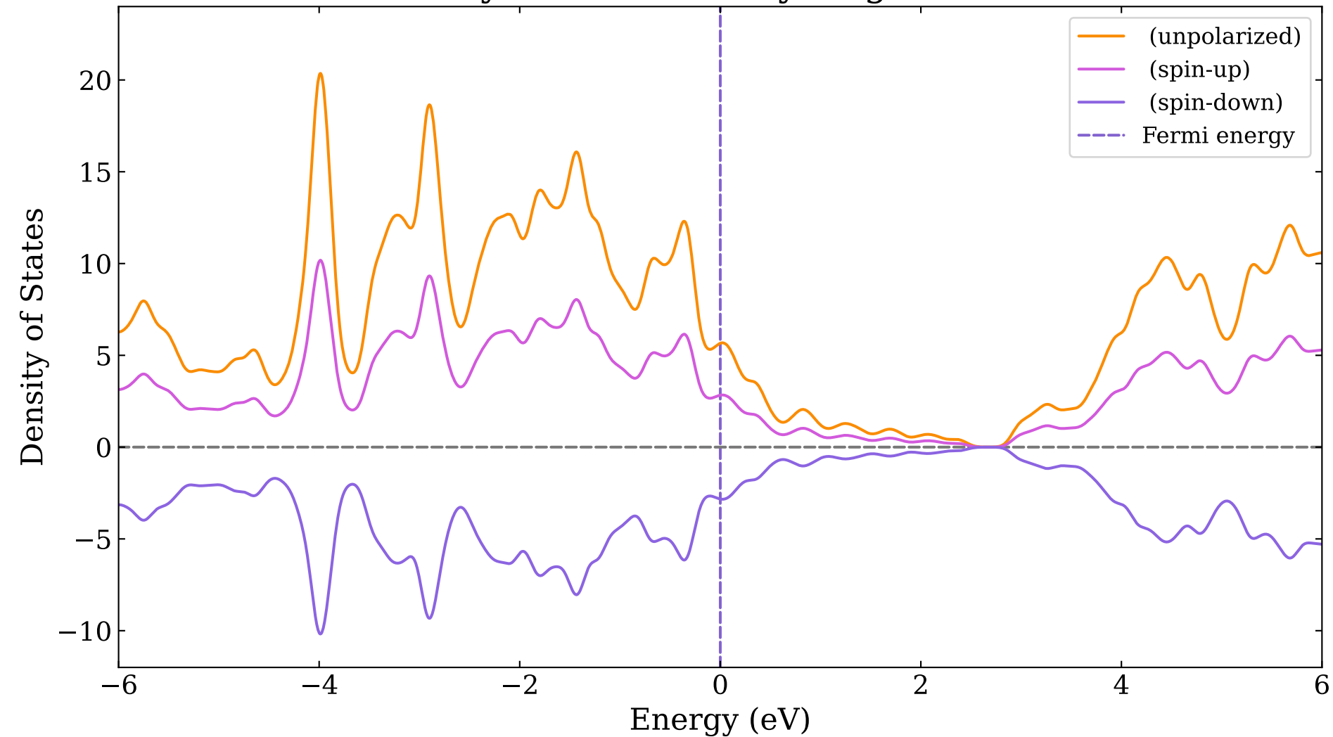
DoS of bilayer o-B 14 with hydrogen termination
