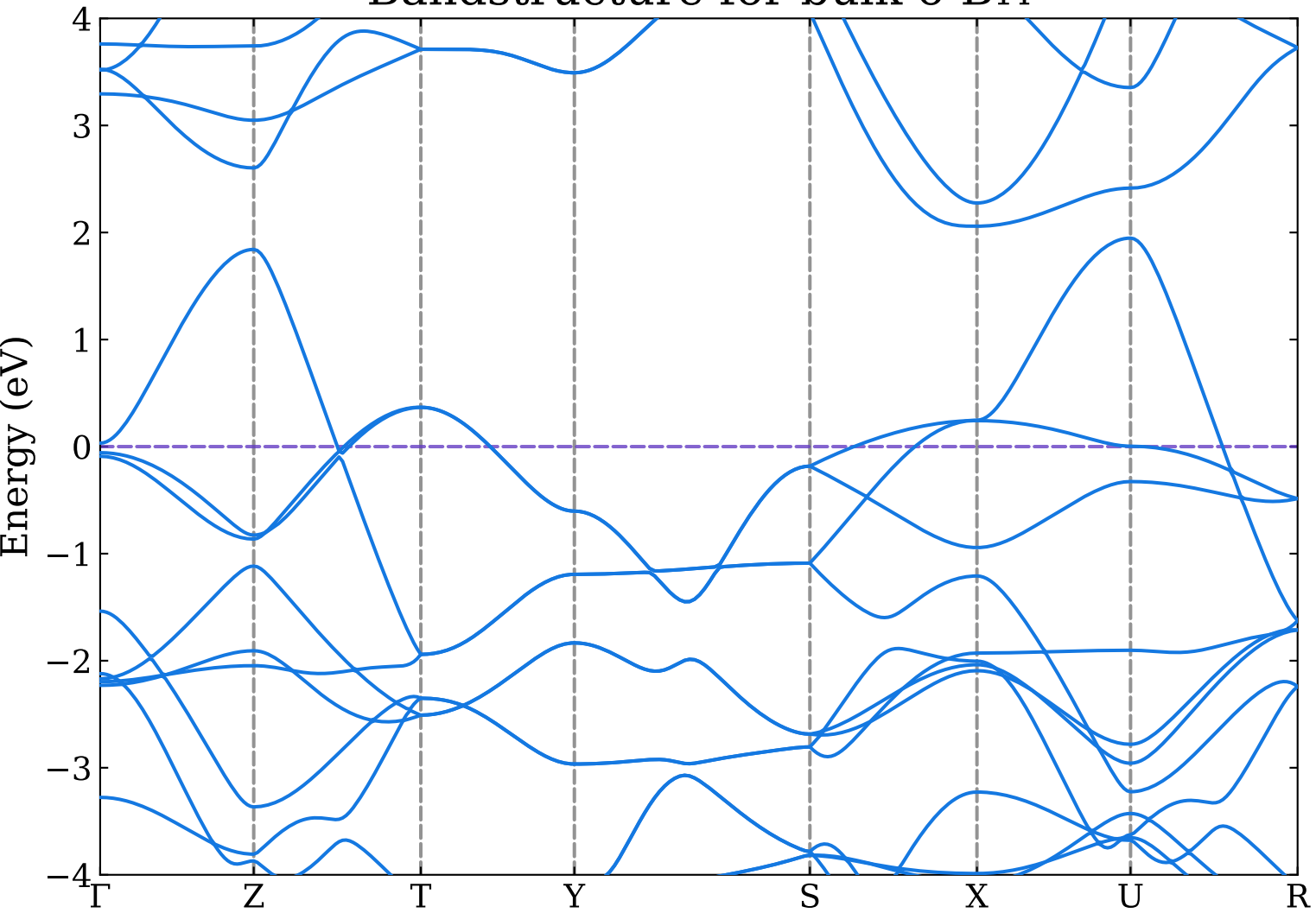
Bandstructure for bulk o-B 14
