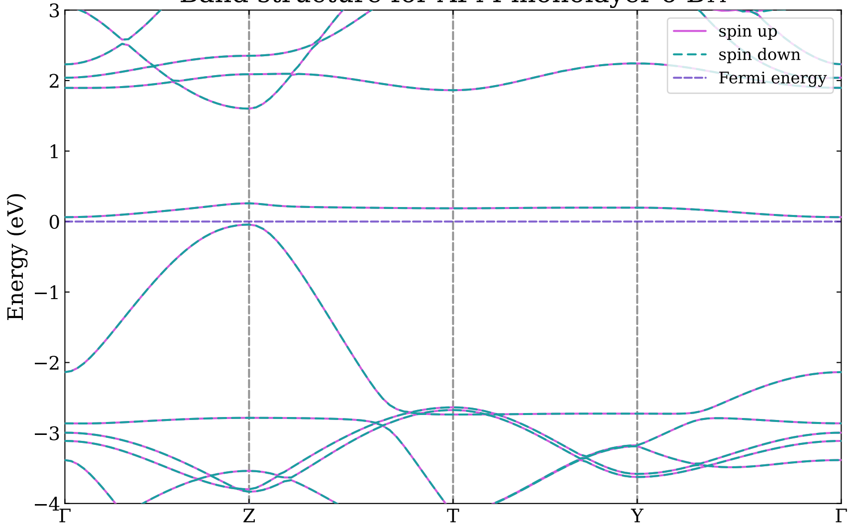
Band structure for AFM monolayer o-B 14
