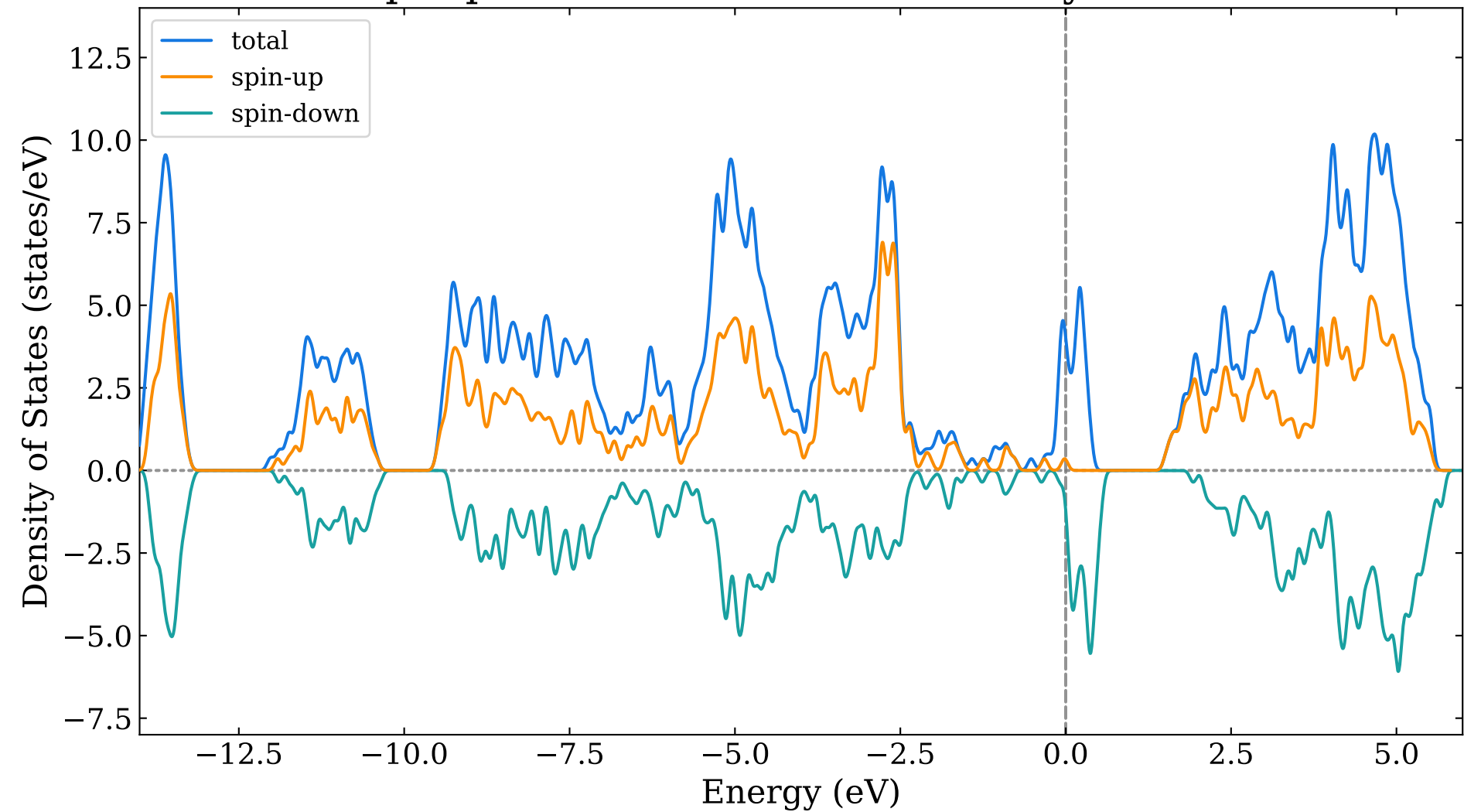
Spin-polarized DoS of FM monolayer o-B 14
