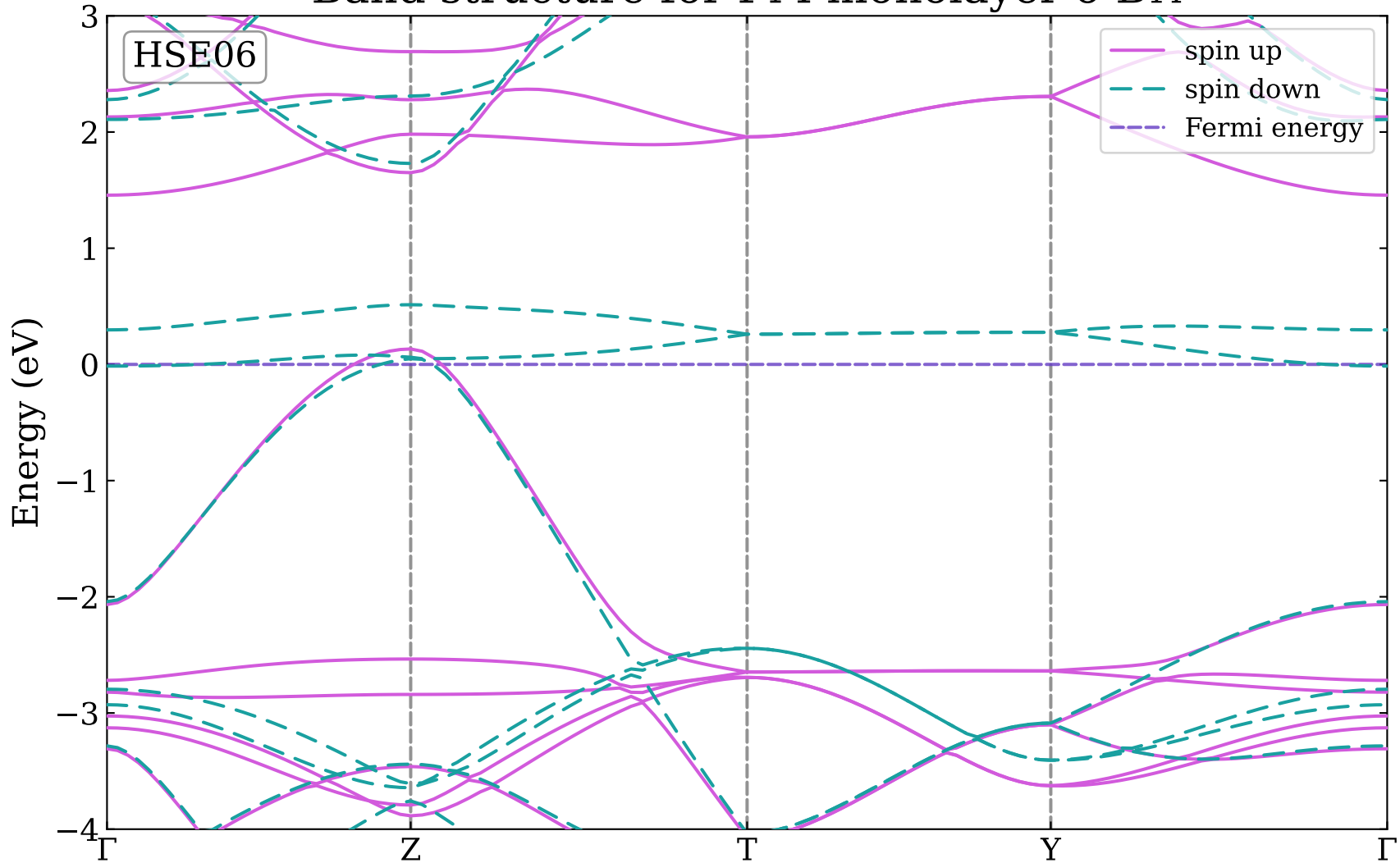
Band structure for FM monolayer o-B 14
