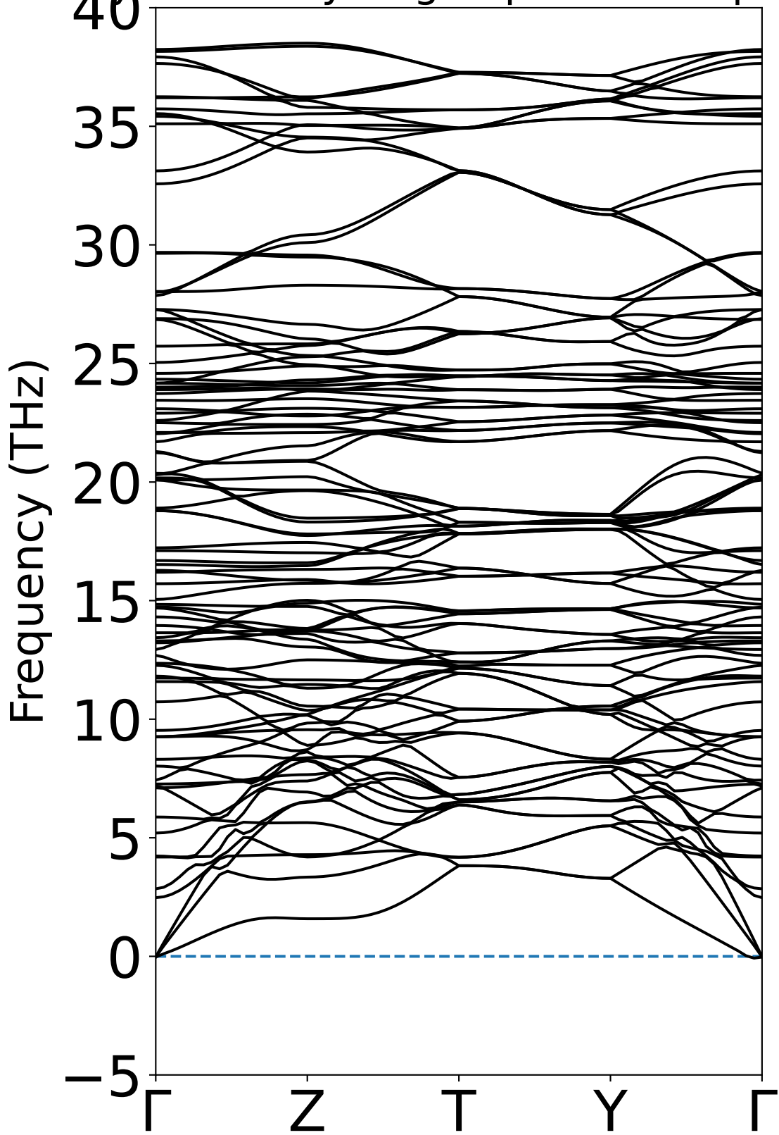
Bilayer with Hydrogen phonon disper
