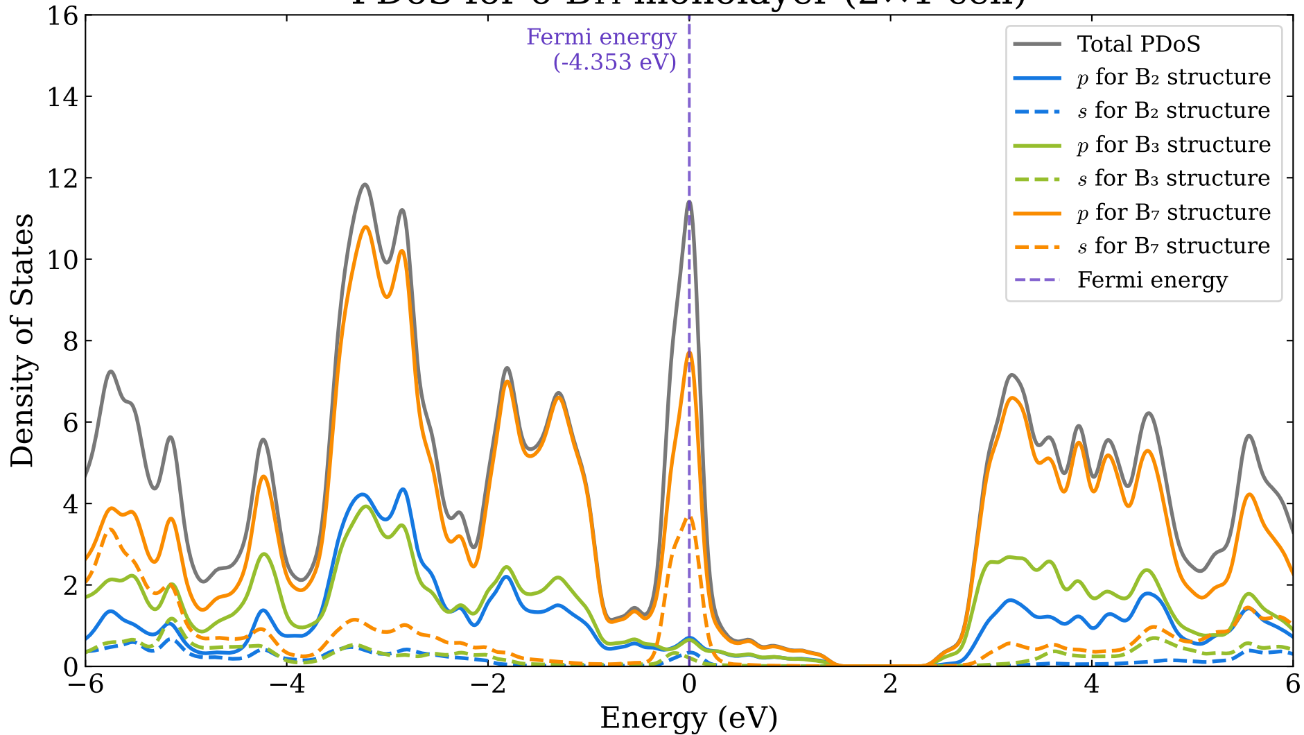
PDoS for o-B 14 monolayer (2×1 cell)
