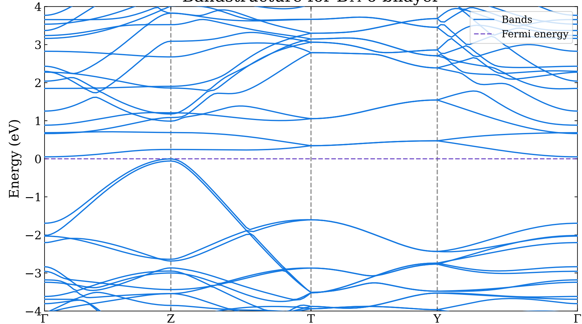
Bandstructure for B 14 o-bilayer
