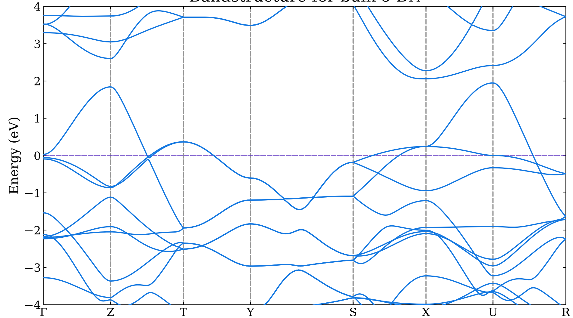
Bandstructure for bulk o-B 14
