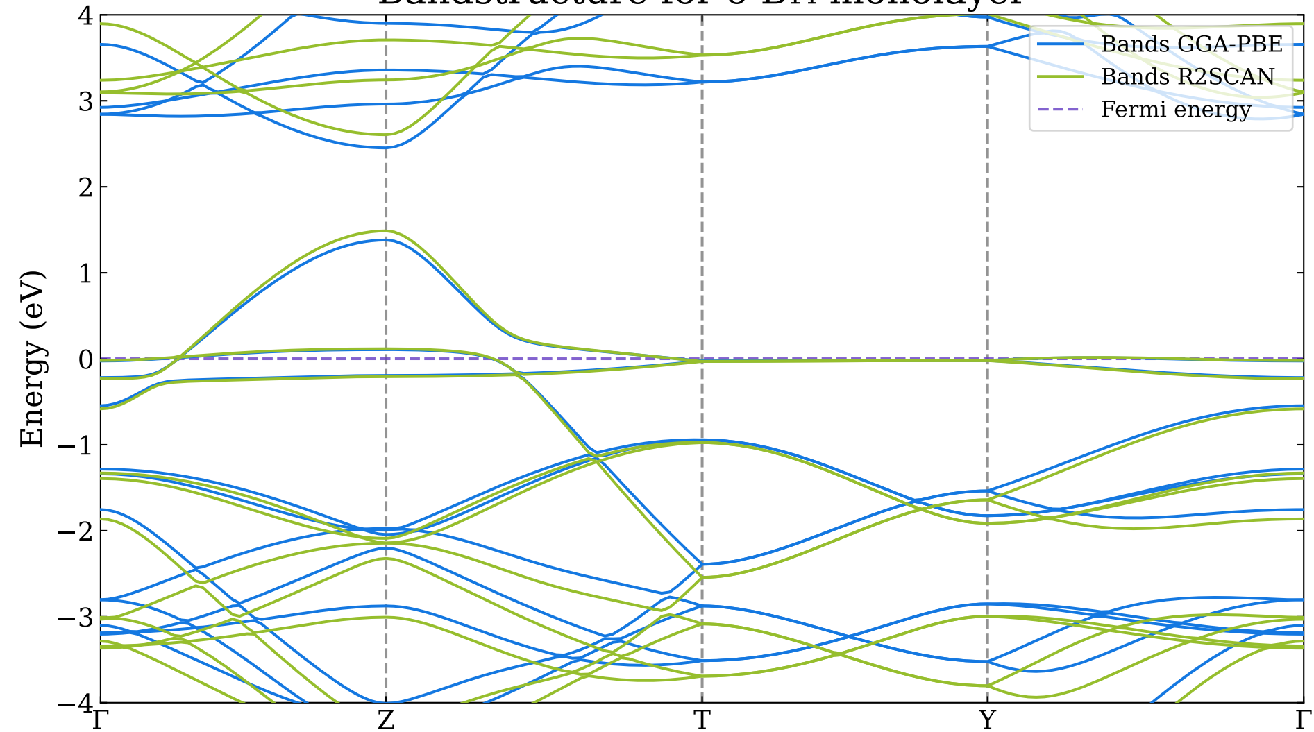
Bandstructure for o-B 14 monolayer
