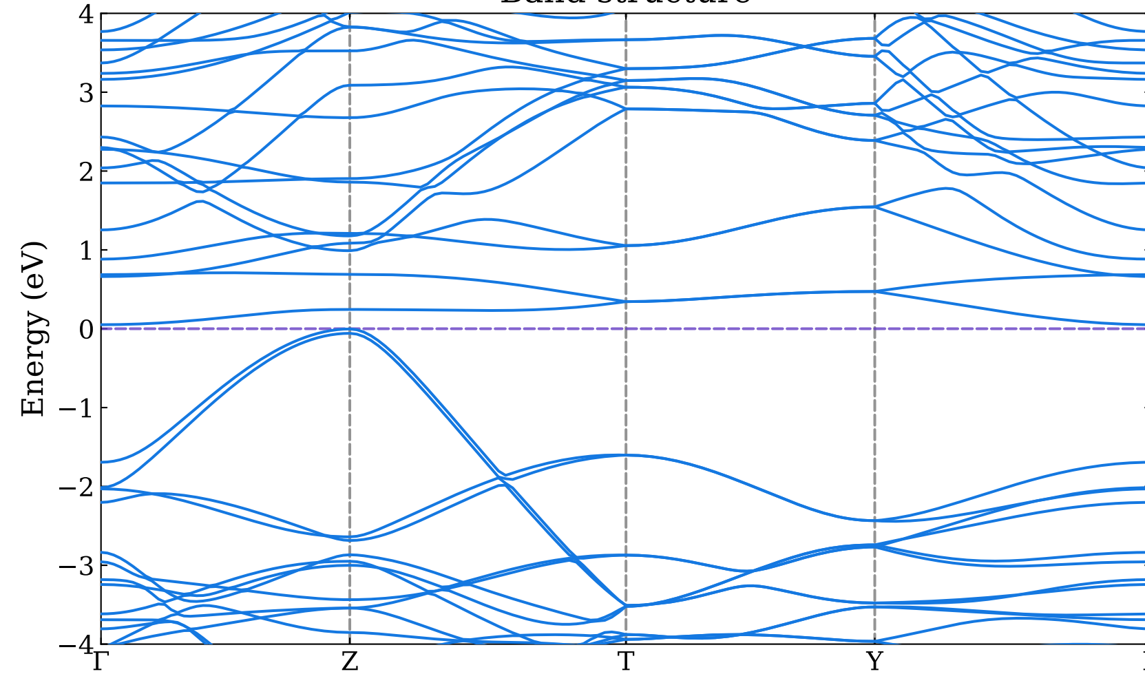
Band structure
