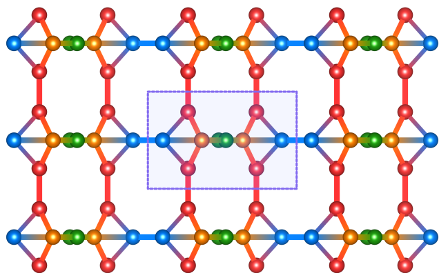
(c) top view of bulk
