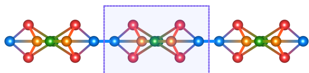
(g) first side view of monolayer
