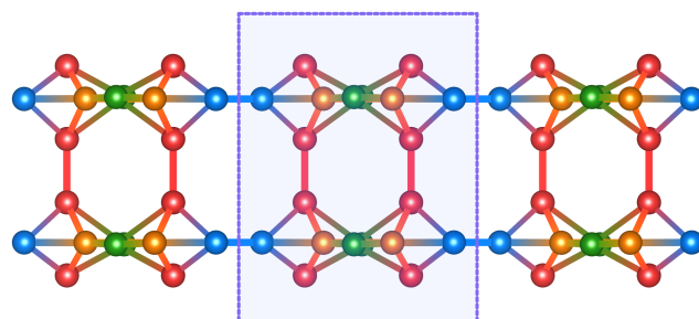
(e) second side view of bilayer
