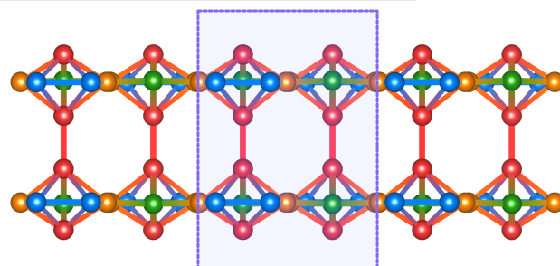
(e) second side view of bilayer
