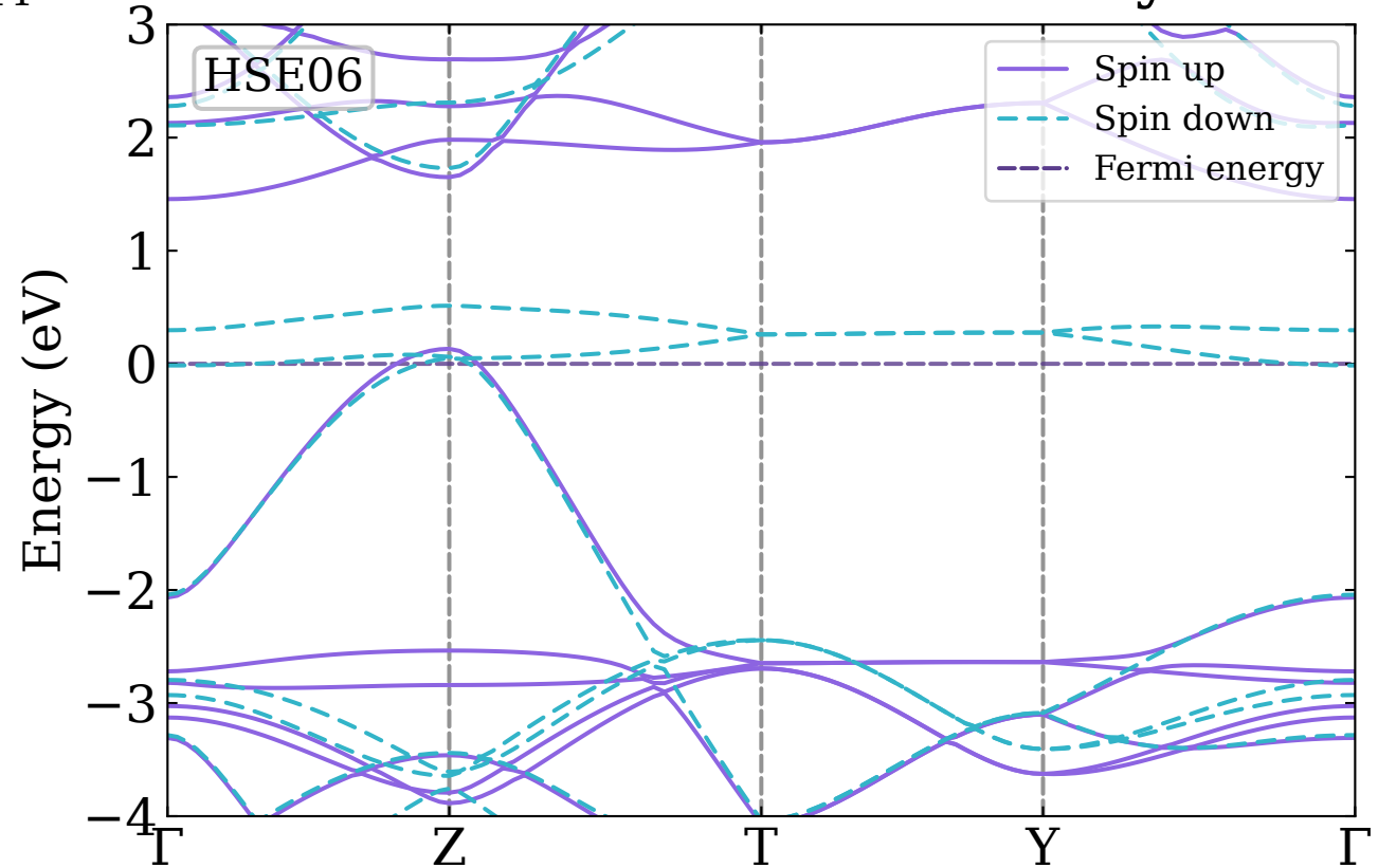
Band structure for FM monolayer o-B 14
