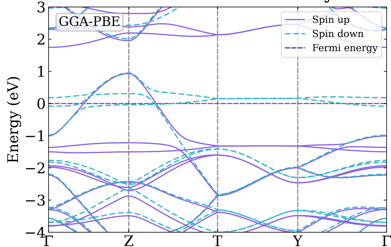
Band structure for FM monolayer o-B 14
