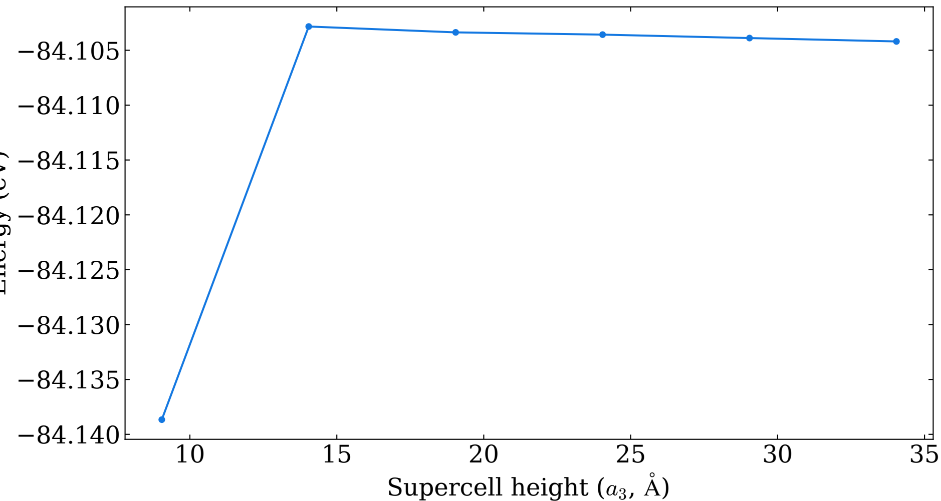
Energy versus supercell height for monolayer o-B 14
