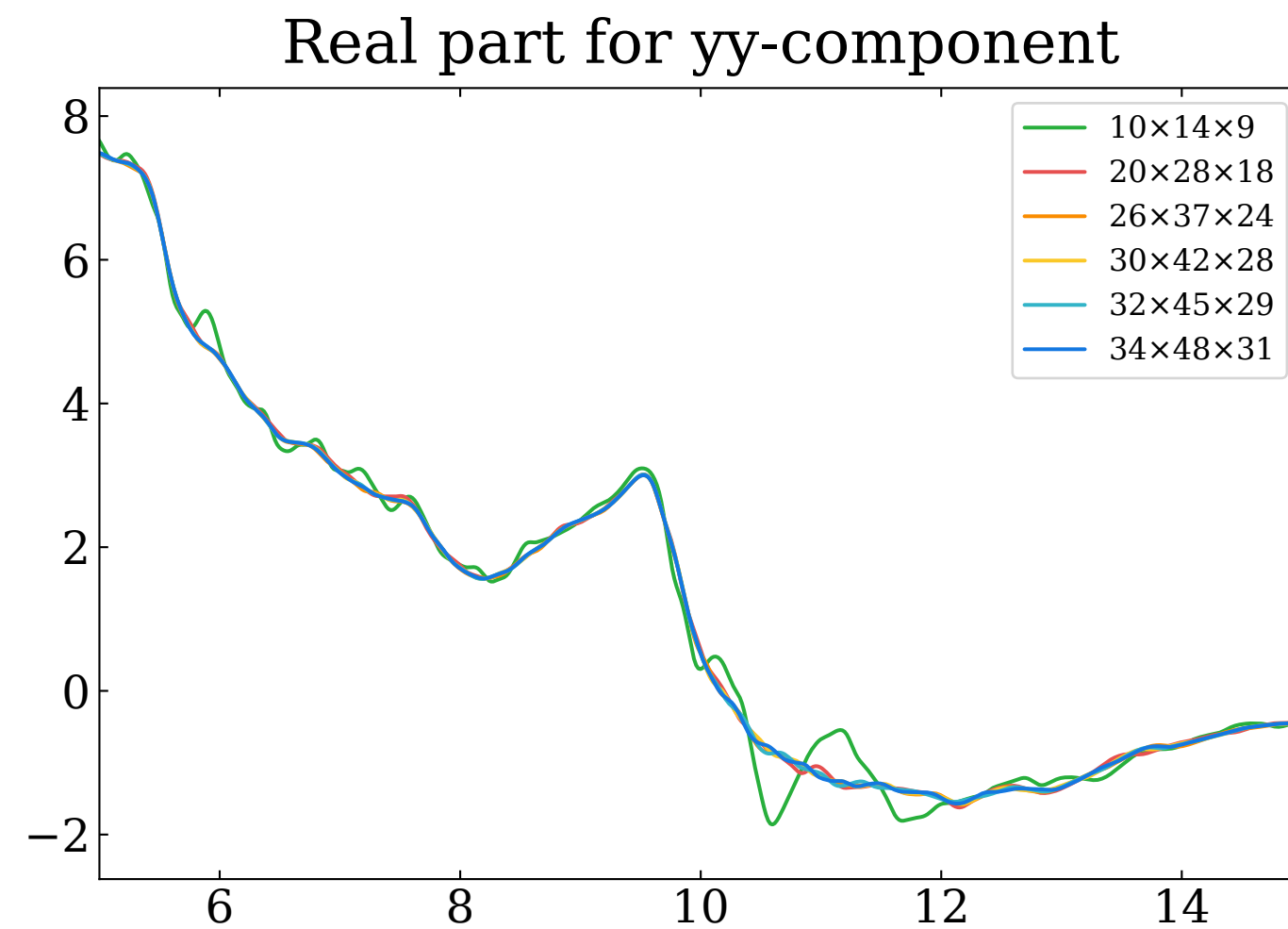
Dielectric function versus k-points for bulk o-B 14
