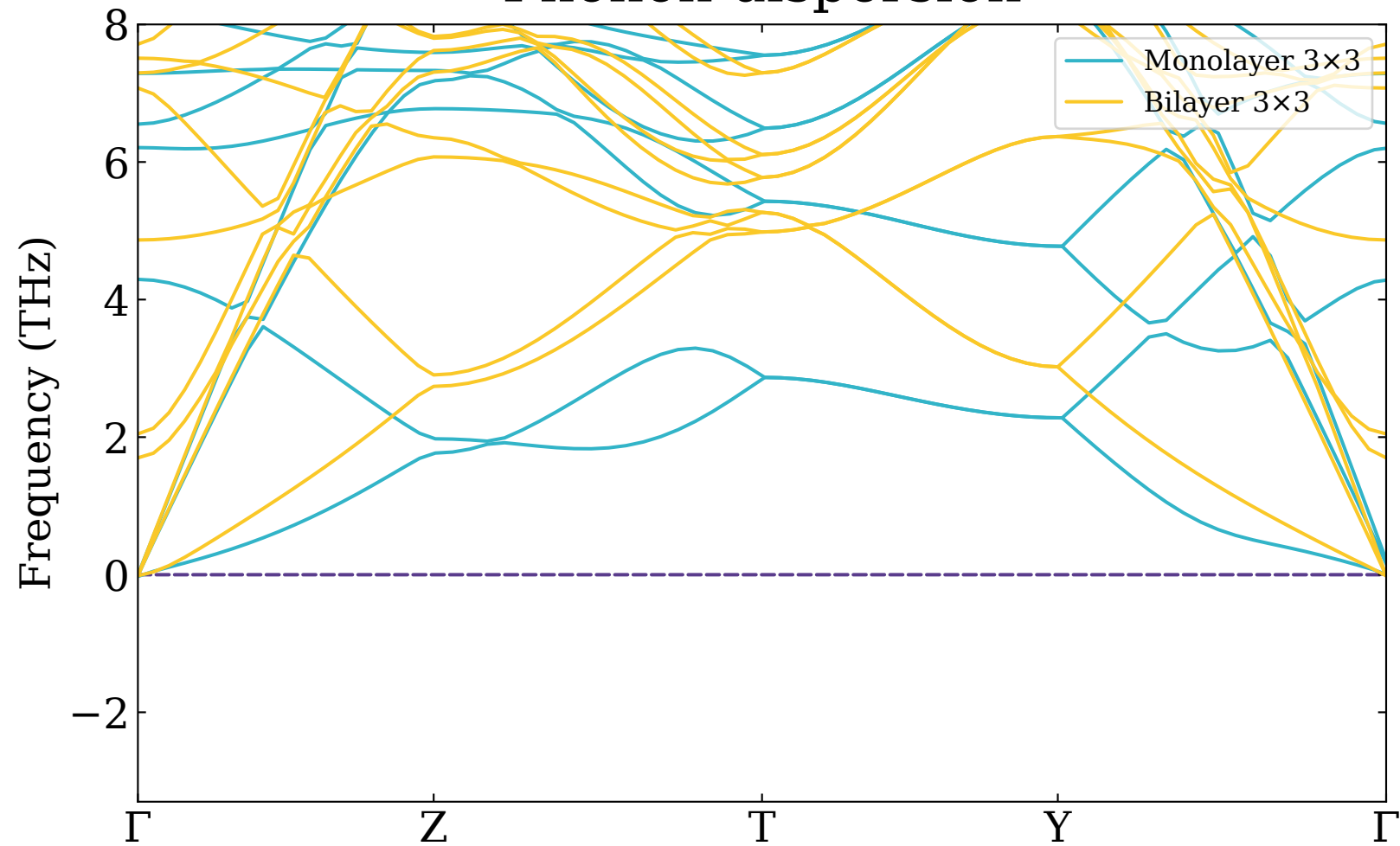
Phonon dispersion
