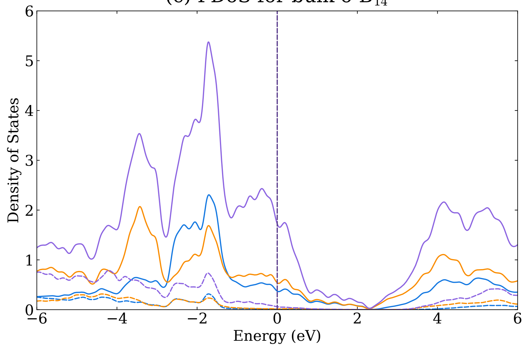
(c) PDoS for bulk o-B 14
