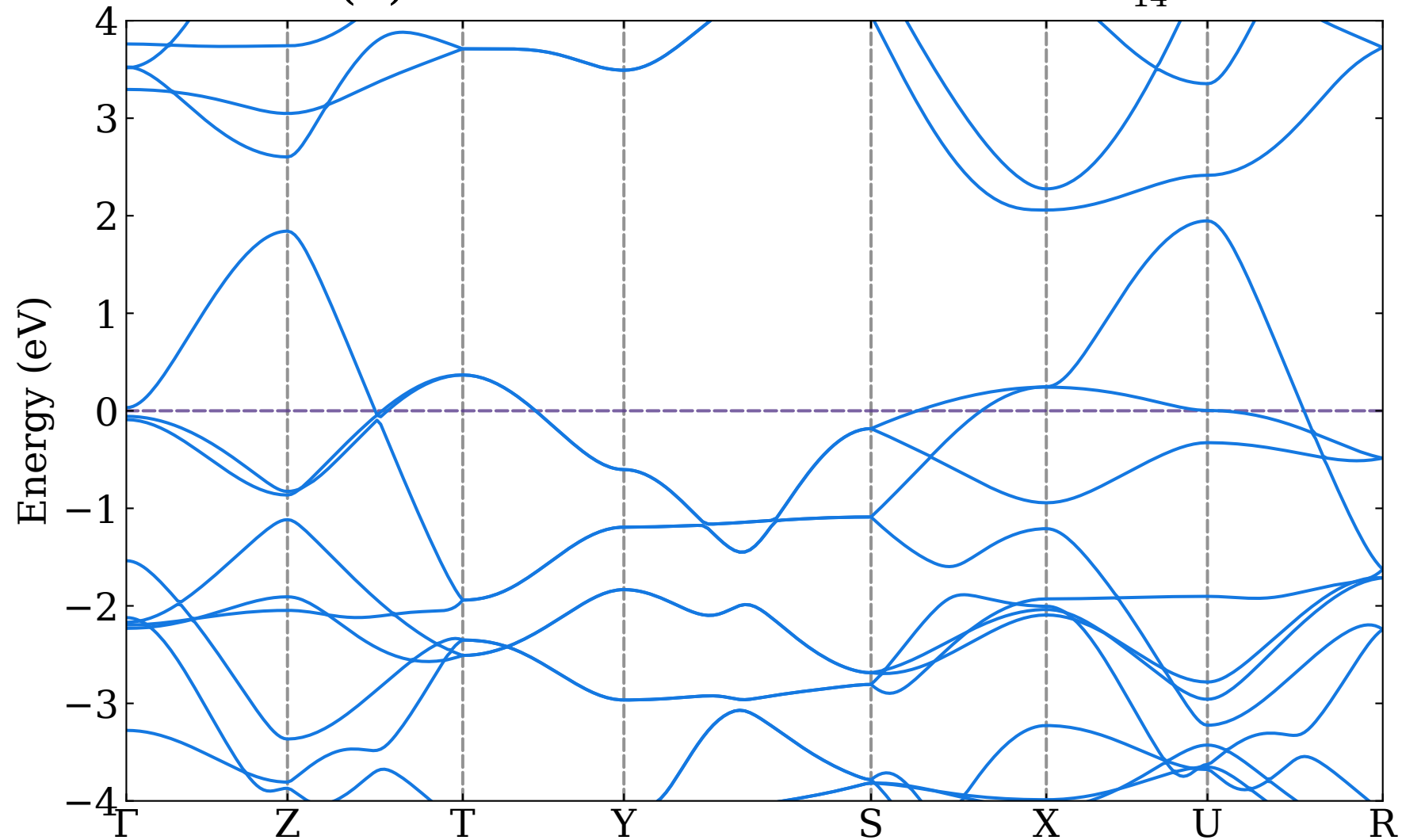
(a) Band structure for bulk o-B 14
