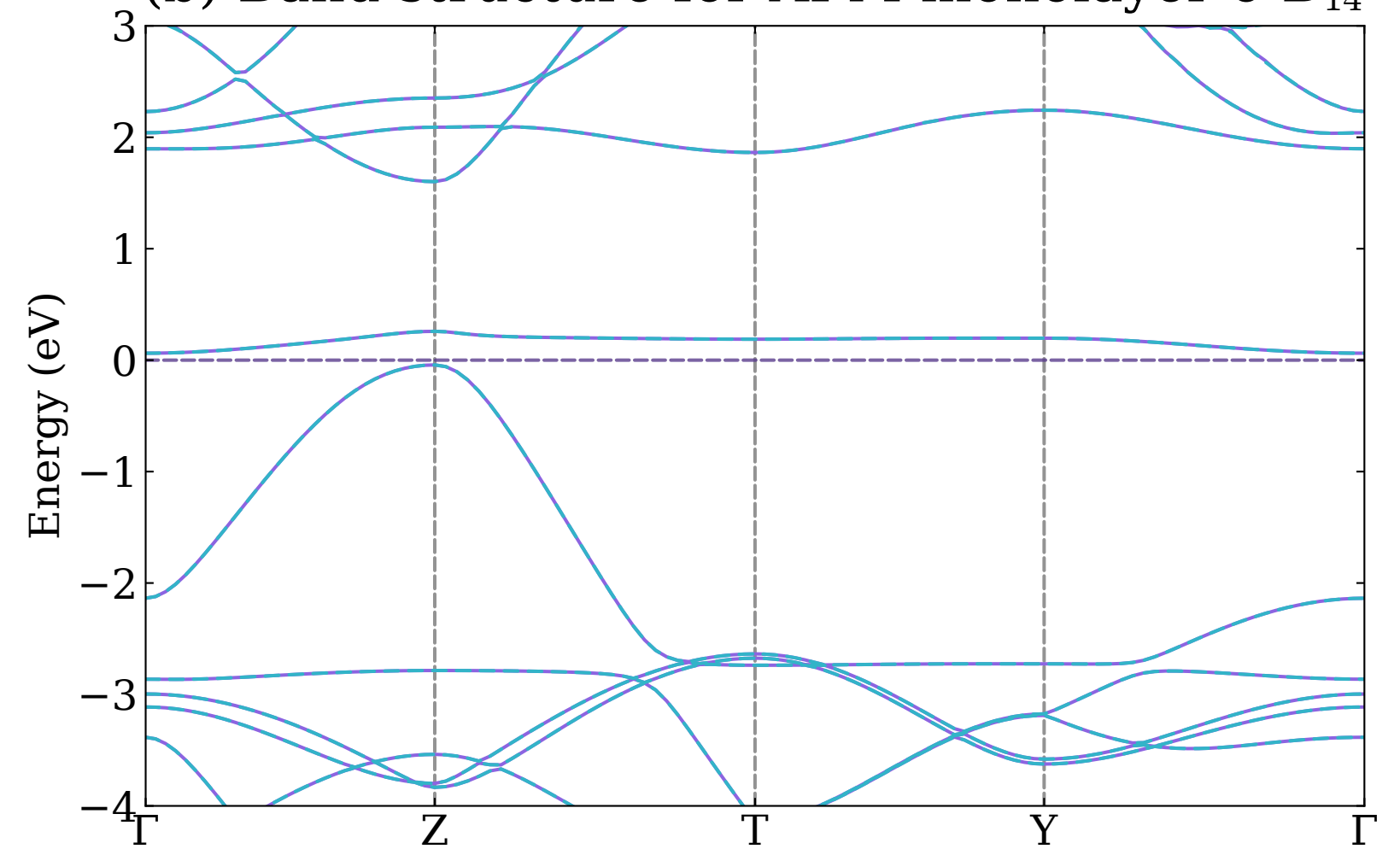
(b) Band structure for AFM monolayer o-B 14
