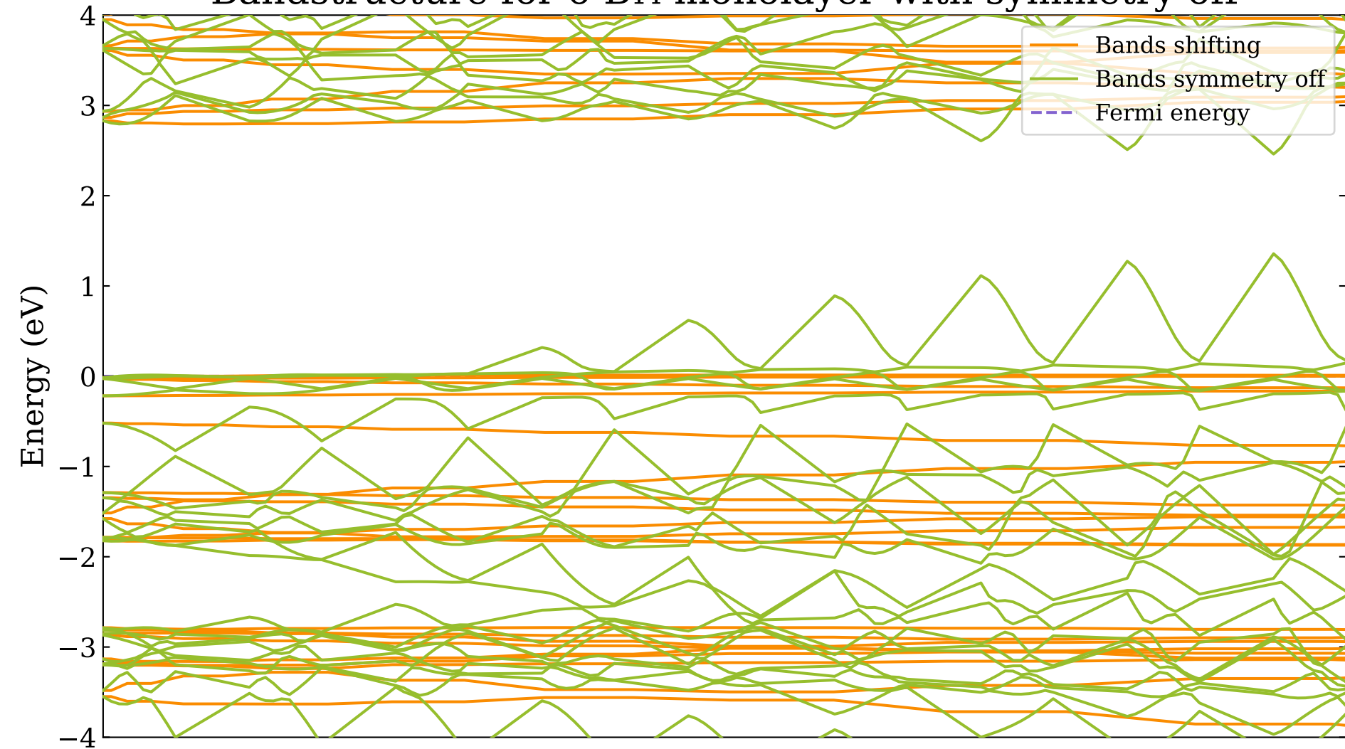
Bandstructure for o-B 14 monolayer with symmetry off
