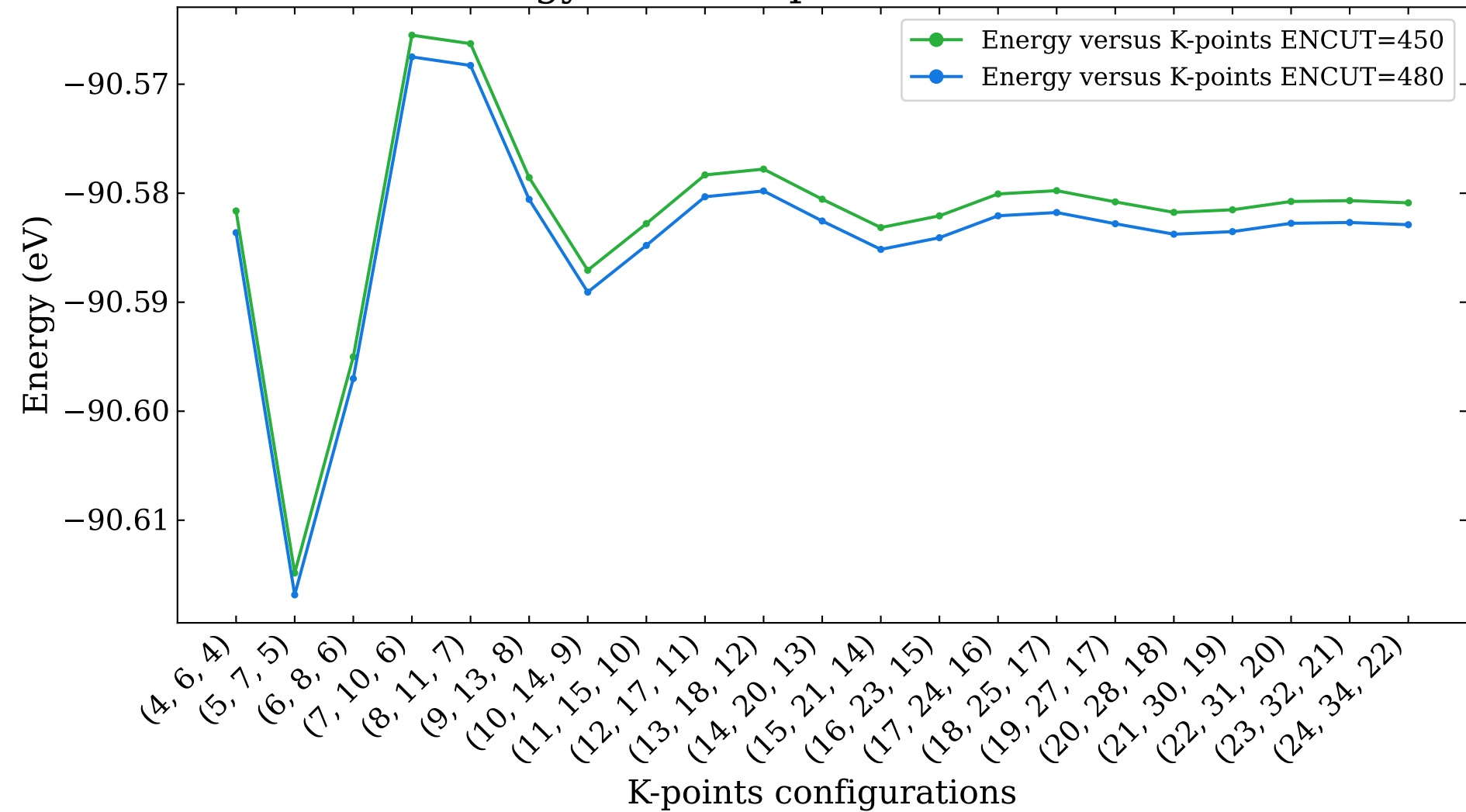
Energy versus K-points for o-B 14 bulk
