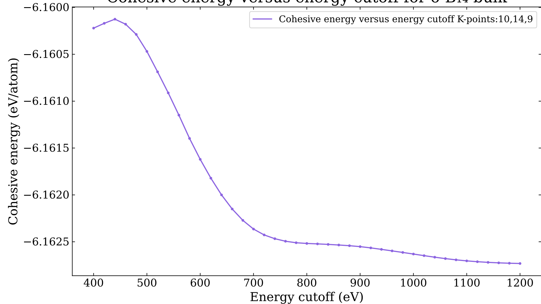
Cohesive energy versus energy cutoff for o-B 14 bulk
