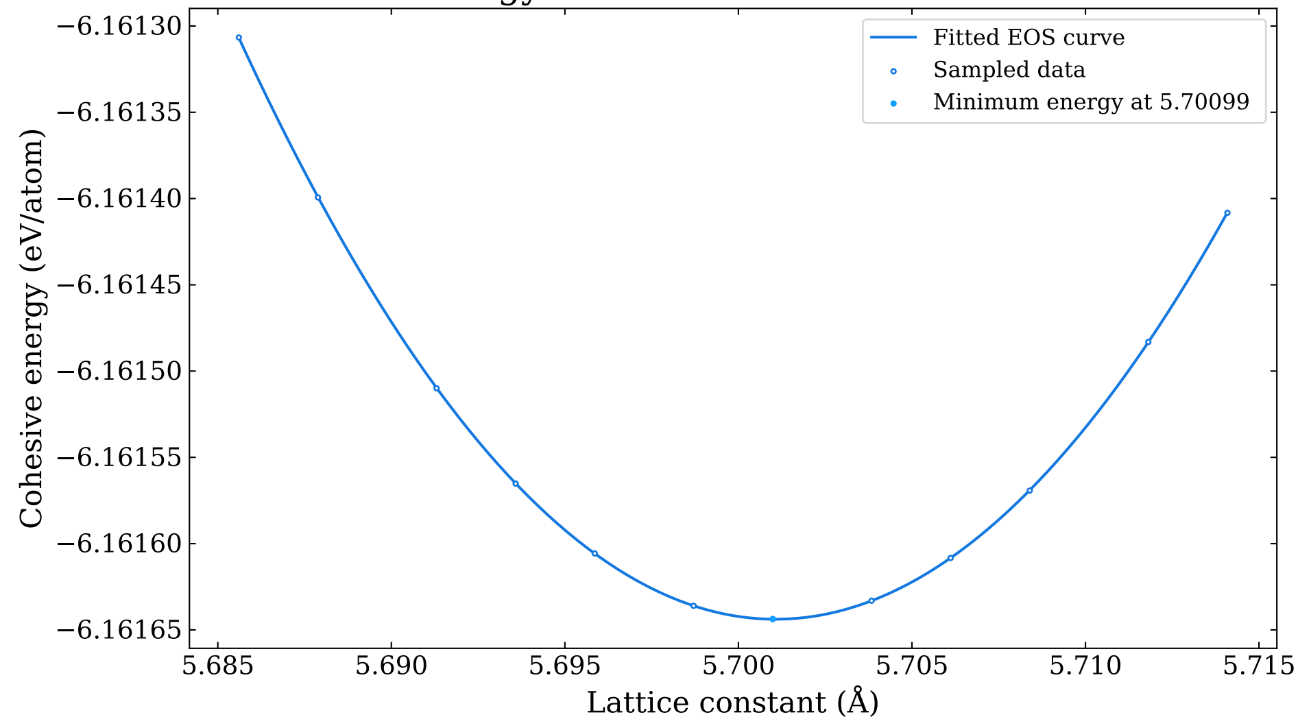
Cohesive energy versus lattice constant for o-B 14 bulk
