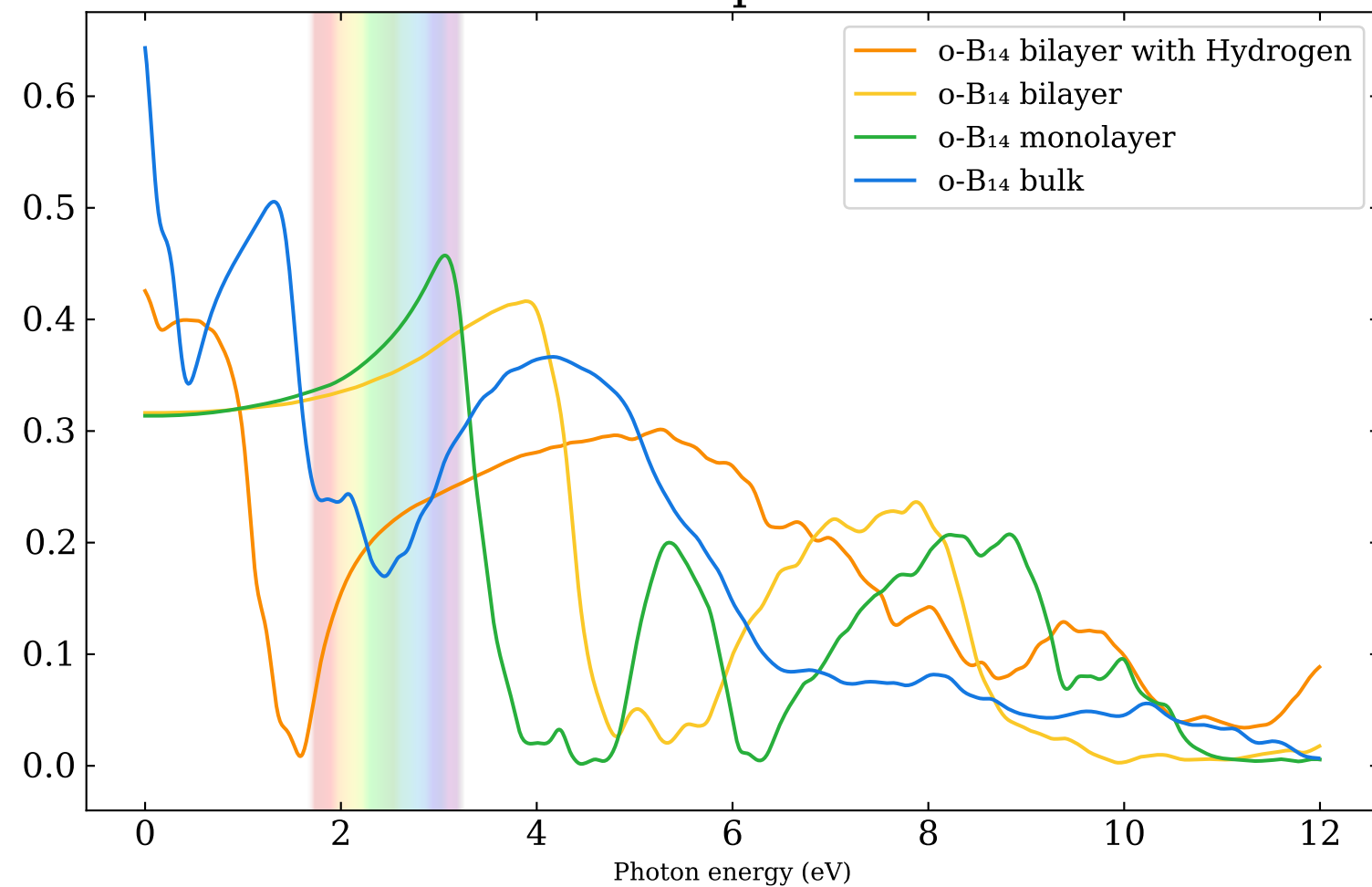
zz-component
