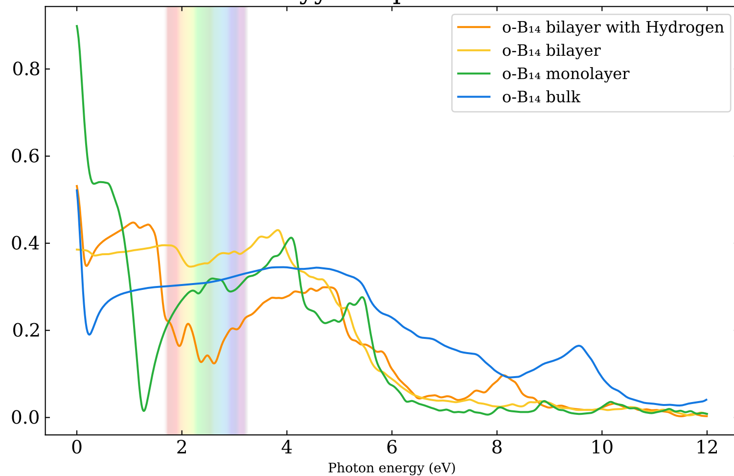
yy-component
