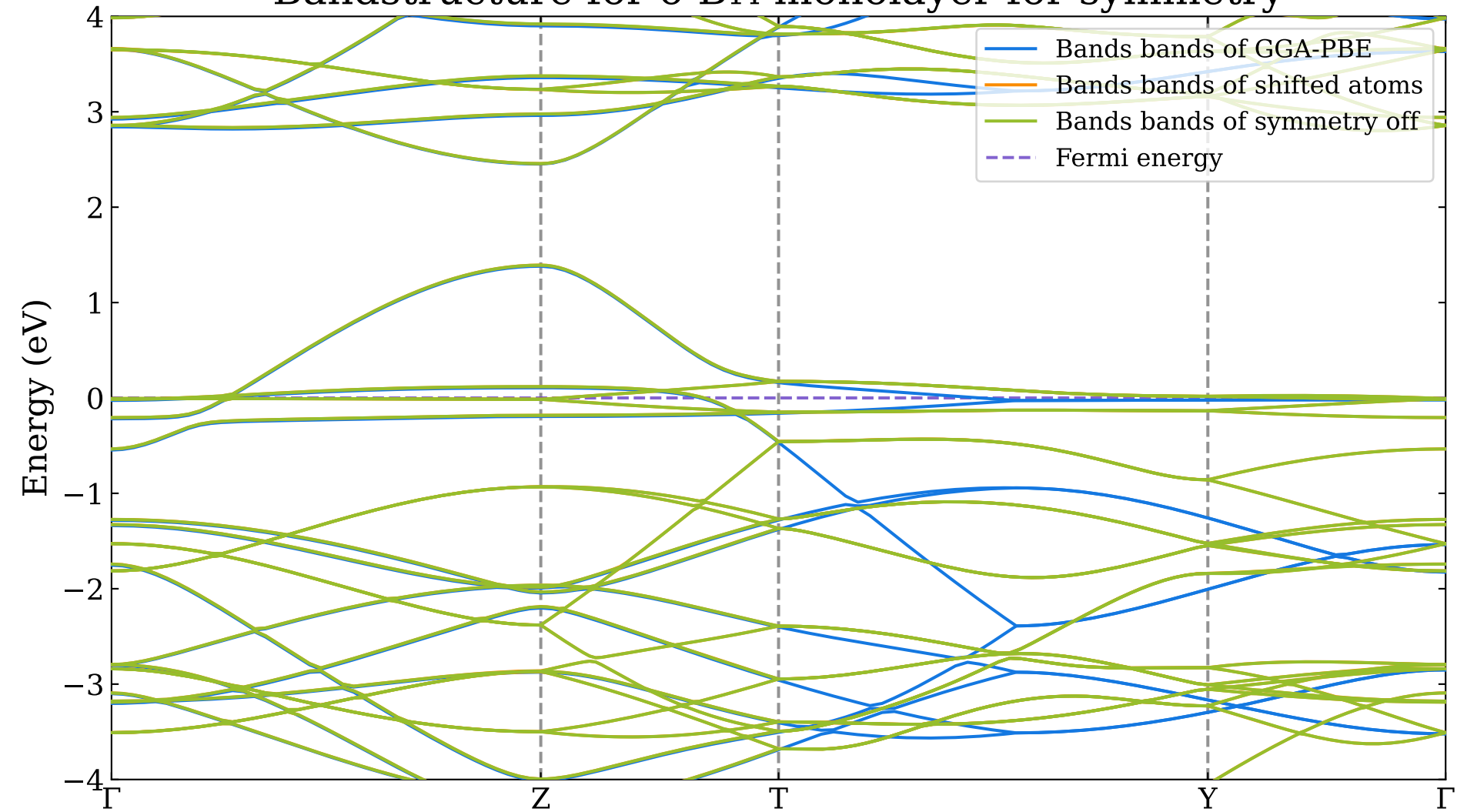
Bandstructure for o-B 14 monolayer for symmetry
