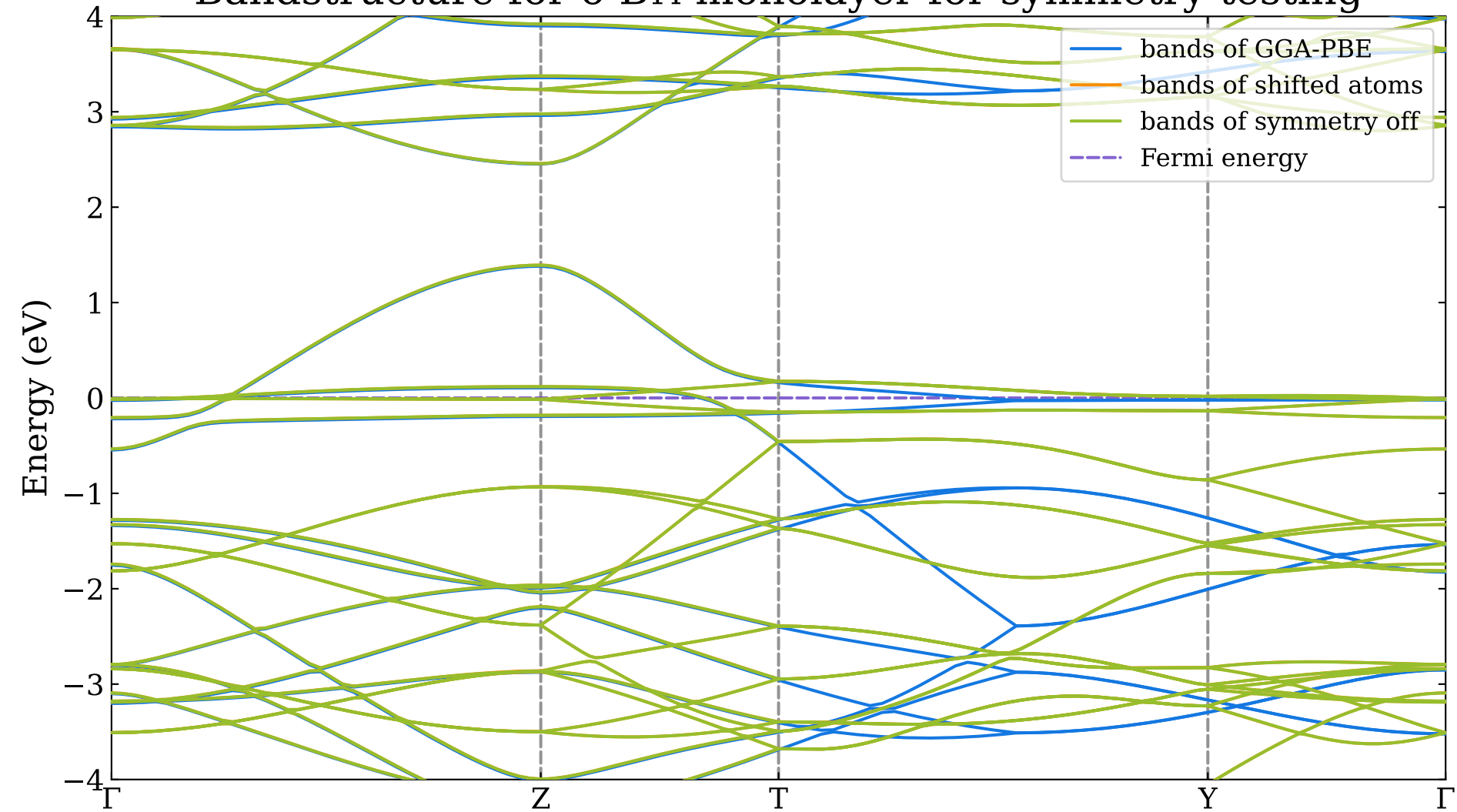
Bandstructure for o-B 14 monolayer for symmetry testing
