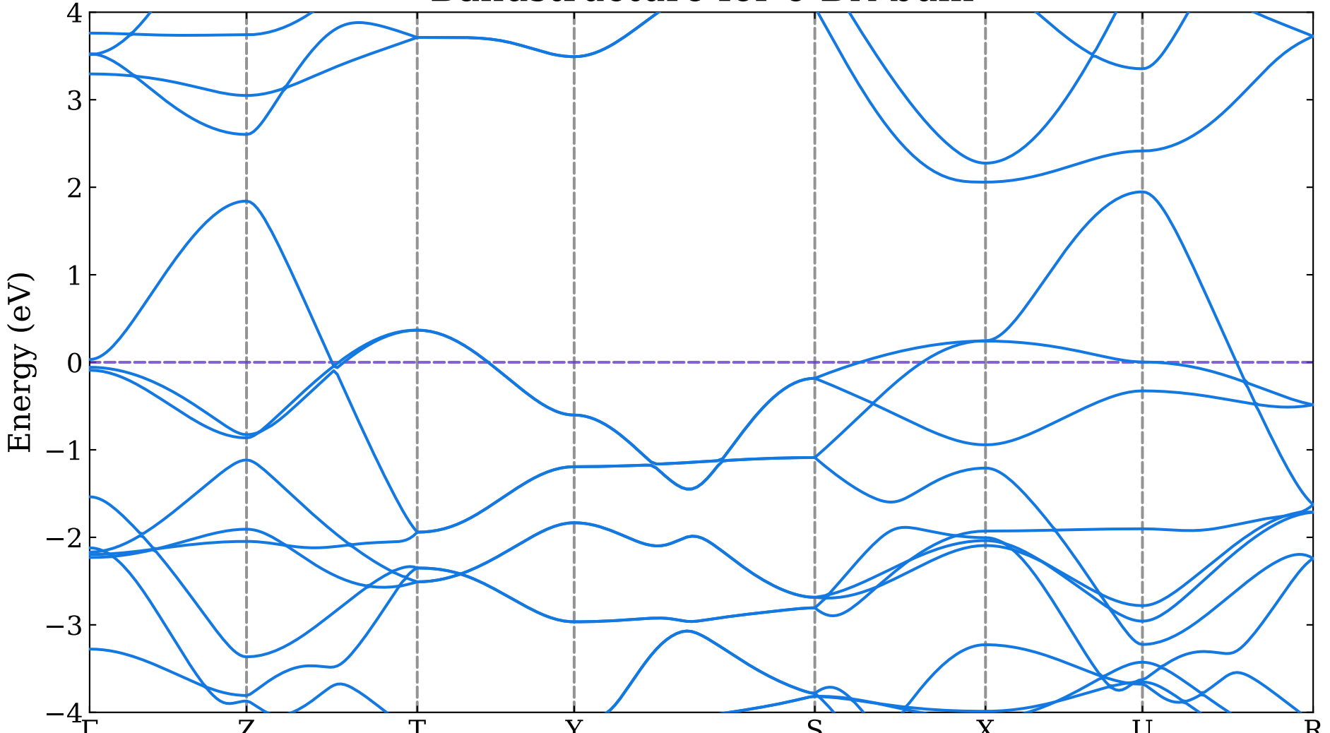
Bandstructure for o-B 14 bulk
