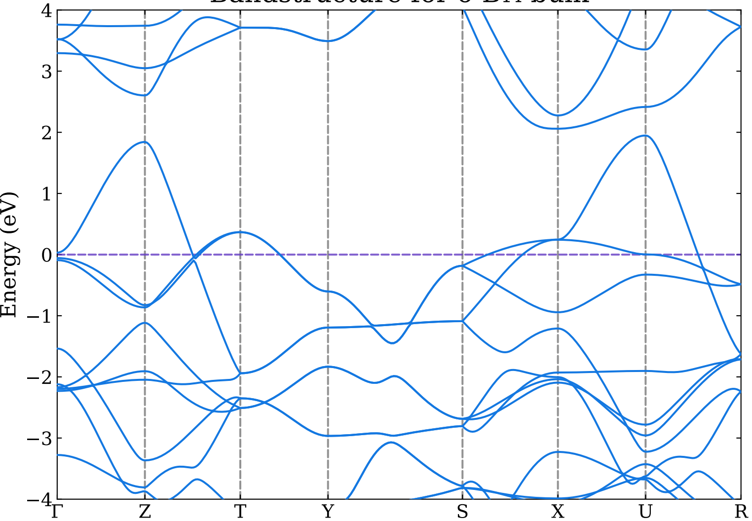
Bandstructure for o-B 14 bulk
