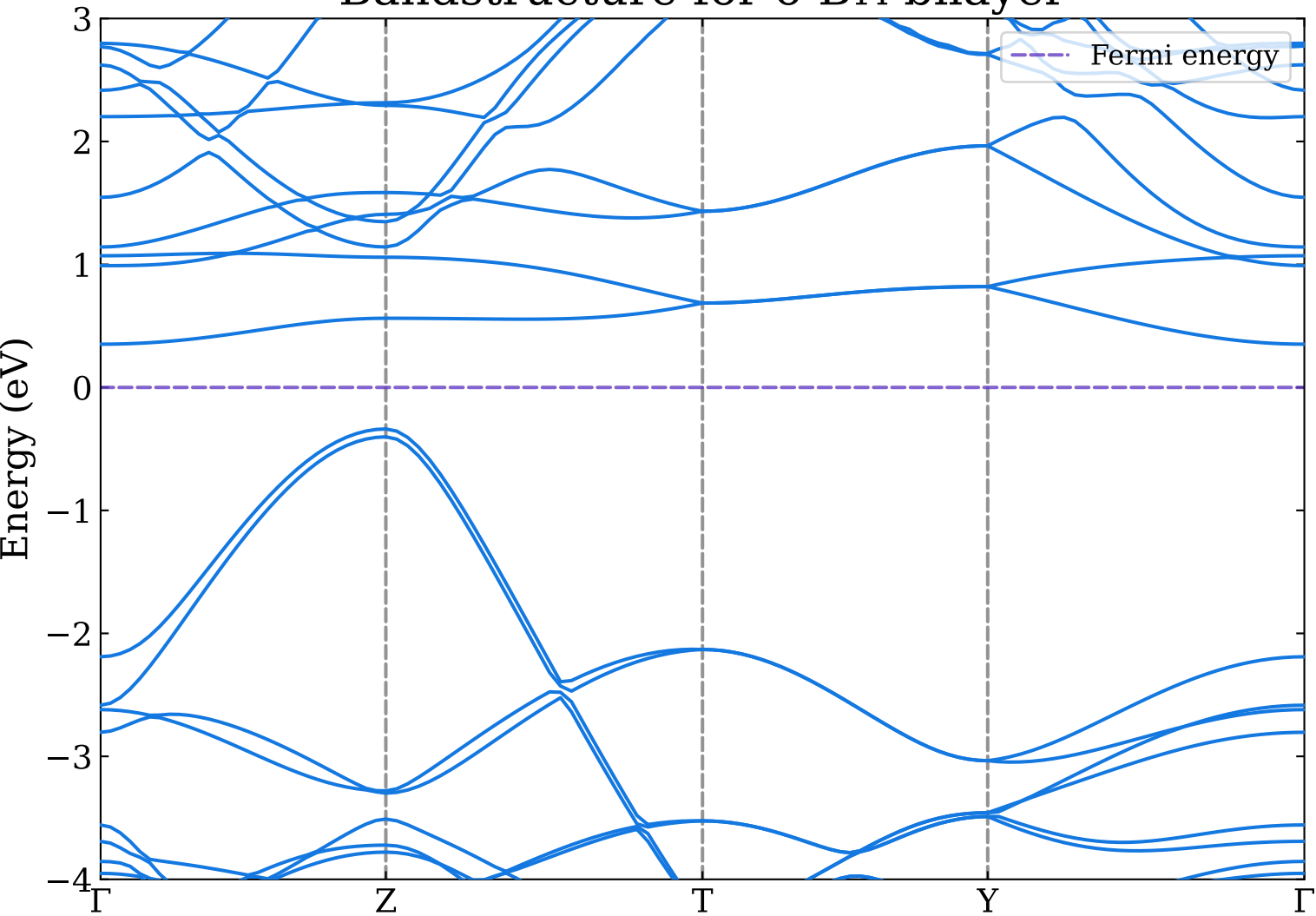
Bandstructure for o-B 14 bilayer
