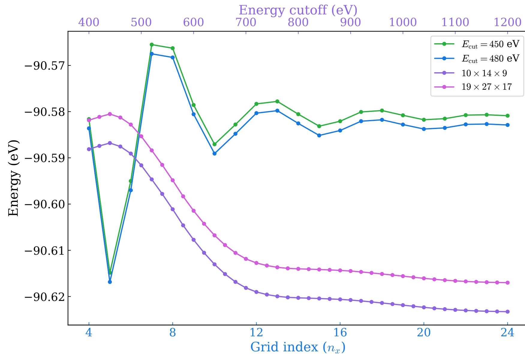
(a) Energy for bulk o-B 14
